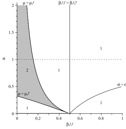
Figure 2: b_1 - b_2 < 0 .
