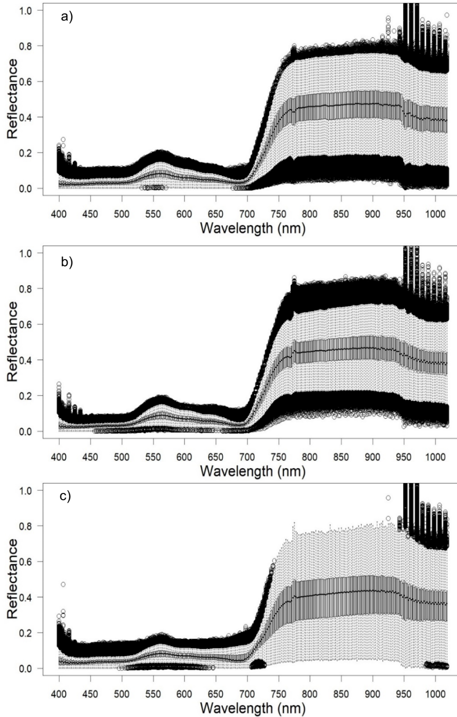
Figure 5. A boxplot visualization of the spectral signatures extracted from the three classes: healthy tree (a), fresh damage (b), and old damage (c). The minimum quartile (0th percentile), the maximum quartile (100th percentile), the first quartile (25th percentile), and the third quartile (75th percentile), and the median (50th percentile) are shown as well as outliers (circles) for each class at each hyperspectral band.
