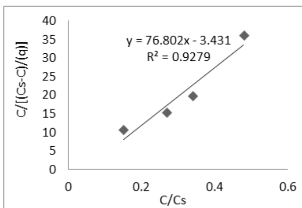
Figure 5. BET adsorption isotherm of Carbaryl on Fe 3 O 4 -CNTs
