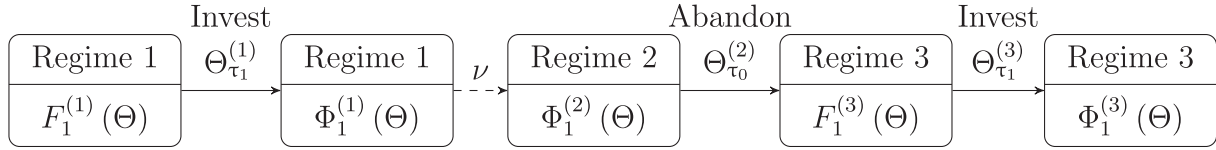
Fig. 1. State-transition diagram.
