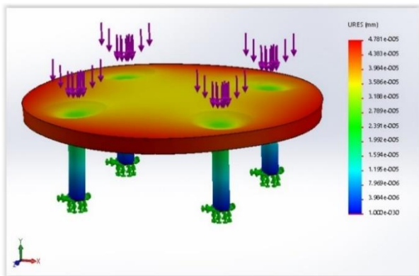
Fig. 28. Displacement of the landing platform.
