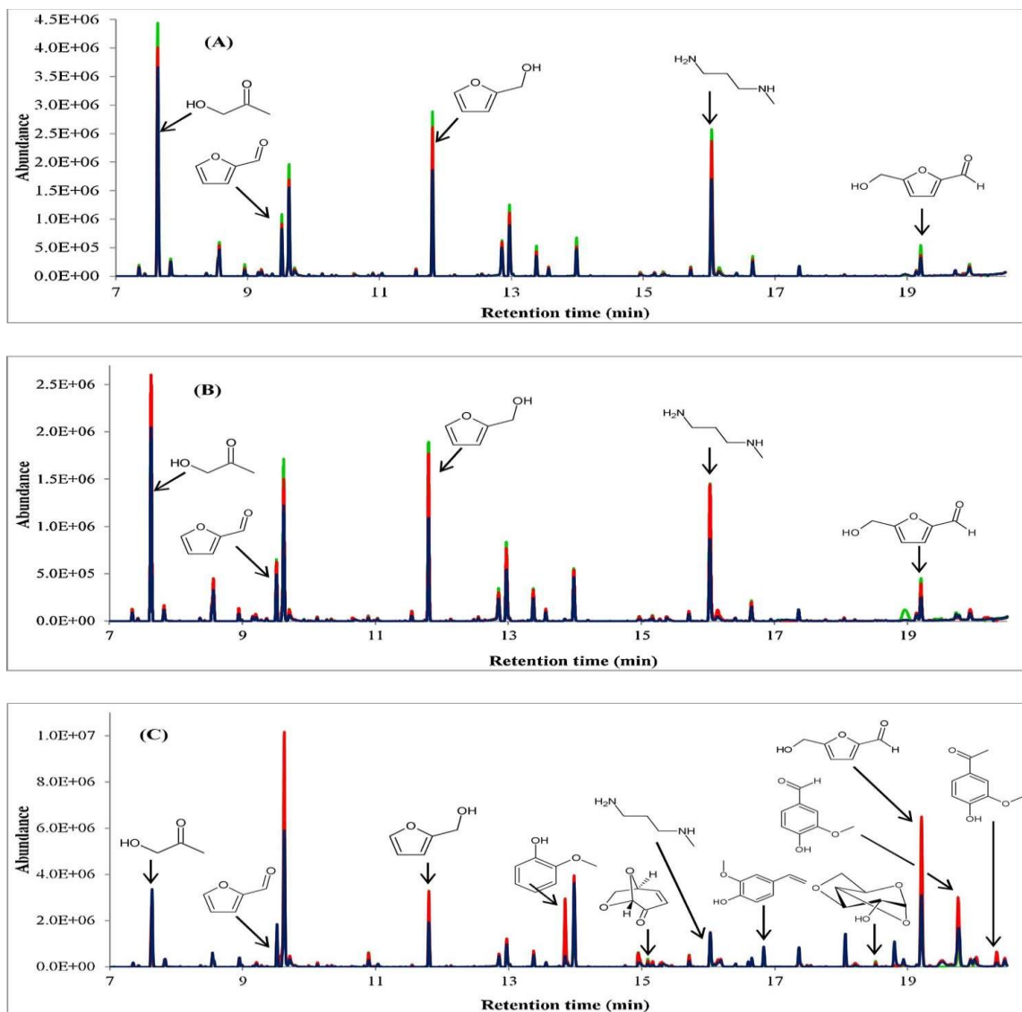
Fig. 1. Pyrolysis products identified in the pyrograms of white (A), notebook (B) and recycled (C) paper, respectively, after an accelerated aging of 475 (green line), 282 (red line) and 2 (blue line) h. Pyrolysis temperature of 400 °C. GC/MS conditions: ZB-WAX column (30 m × 0.25 mm × 0.25 μm), split injection (1:10), injection temperature of 300 °C, temperature gradient: 40 °C hold for 2 min, 12 °C min -1 to 250 °C, 250 °C hold for 1 min (For interpretation of the references to colour in this figure legend, the reader is referred to the web version of this article.)
