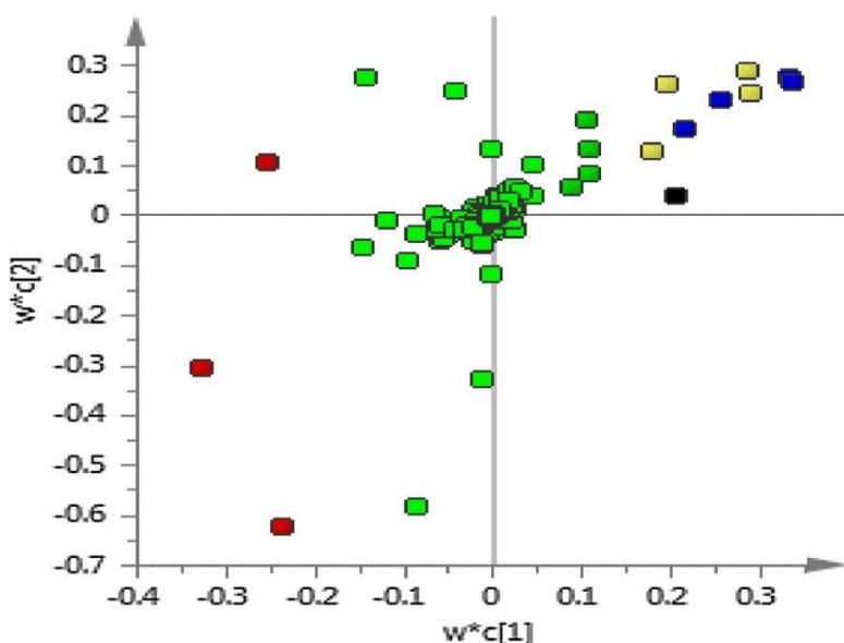
Fig. 3. Loadings Plot of the PLS model applying SNV filter. The first factor ( R^2X 20.7%) was represented against the second factor ( R^2X 62.3%). The green and black points represent the variables X and Y, respectively. The variables X ( t_R ) corresponding to 2-furanmethanol and N-methyl-3-propanediamine are specified by the yellow and blue points, respectively while 1-hydroxy-2-propanone is characterized by the red ones. (For interpretation of the references to colour in this figure legend, the reader is referred to the web version of this article.)
