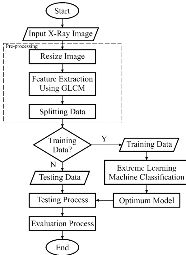
Figure 3. COVID-19 Detection using GLCM-ELM Flowchart
