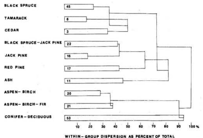
FIGURE 2 SUMMARY DENDROGRAM
