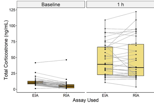
Figure 2: Comparison of EIA and RIA results for quantifying total plasma CORT concentration in B. irregularis collected in 2018 immediately after capture (baseline) and after snakes were subjected to acute confinement in a cloth bag for 1 h. Box plots depict the minimum, first quartile, median, third quartile and maximum. Individual points represent samples. Lines connect aliquots of the same sample. Values shown are untransformed.
