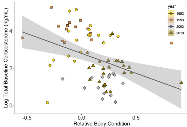
Figure 3: Log total baseline plasma CORT (measured by RIA) was negatively associated with relative body condition in B. irregularis on Guam in all years except 1992. CORT was higher and Body condition was lower in 1992 and 1993 compared with 2003 and 2018. Shaded area represents the 95% confidence interval.
