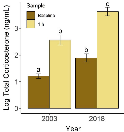
Figure 4: Log total plasma CORT of B. irregularis measured by RIA immediately after capture (baseline, dark shading) and after snakes were subjected to acute confinement in a cloth bag for 1 h (light shading) in 2003 and 2018. Letters indicate significantly different groups.
