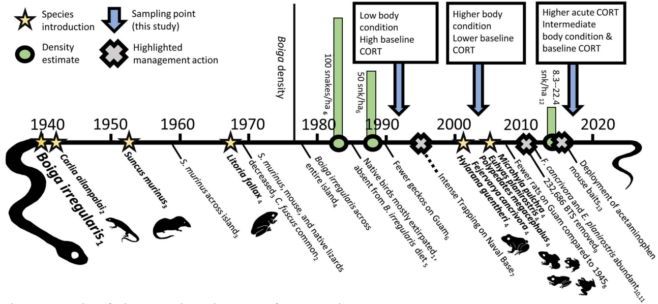
Figure 1: Timeline of select events during the invasion of B. irregularis on Guam. Population estimates are for Northern Guam, where the majority of sampling for this study took place. Subscripts indicate source(s) of information. Note that estimates of snake density should be interpreted with caution, as studies may not be directly comparable due to different methods. Introduction dates are estimates based on the literature. References: (i) Savidge, 1987; (ii) Austin et al. , 2011; (iii) Fritts and Rodda, 1998; (iv) Christy et al. , 2007a; (v) Savidge, 1988; (vi) Rodda et al. , 1992; (vii) Engeman 1998; (viii) Wiewel et al. , 2009; (ix) Engeman et al. , 2018; (x) Wostl et al. , 2016; (xi) Olson et al. , 2012; (xii) Smith et al. , 2016; (xiii) Siers et al. , 2018.
