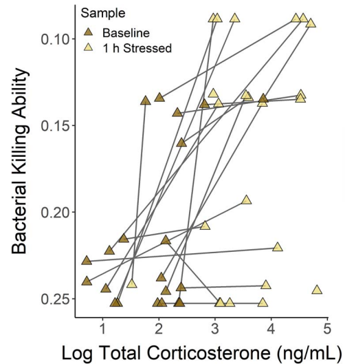
Figure 5: Bacterial killing ability (the arcsine transformed dilution of plasma required to kill 50% of bacteria) was positively related to log total plasma CORT levels in B. irregularis (measured by RIA) sampled in 2018, such that higher CORT was associated with better bacterial killing ability. Blood samples were drawn immediately after capture (baseline, dark shading) and after snakes were subjected to acute confinement in a cloth bag for 1 h (light shading). Letters indicate significantly different groups.
