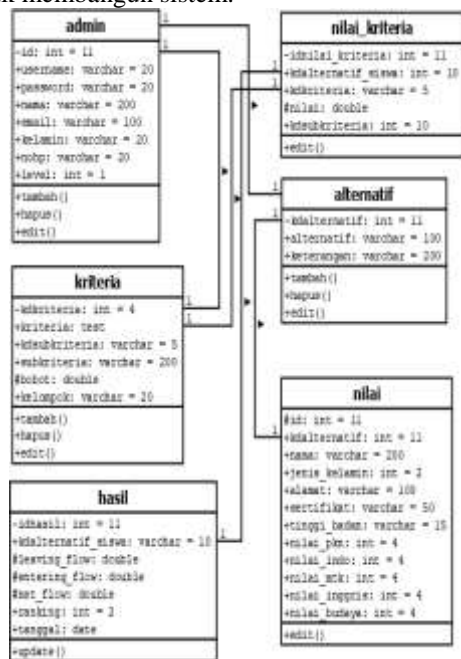
Gambar 9. Class Diagram
