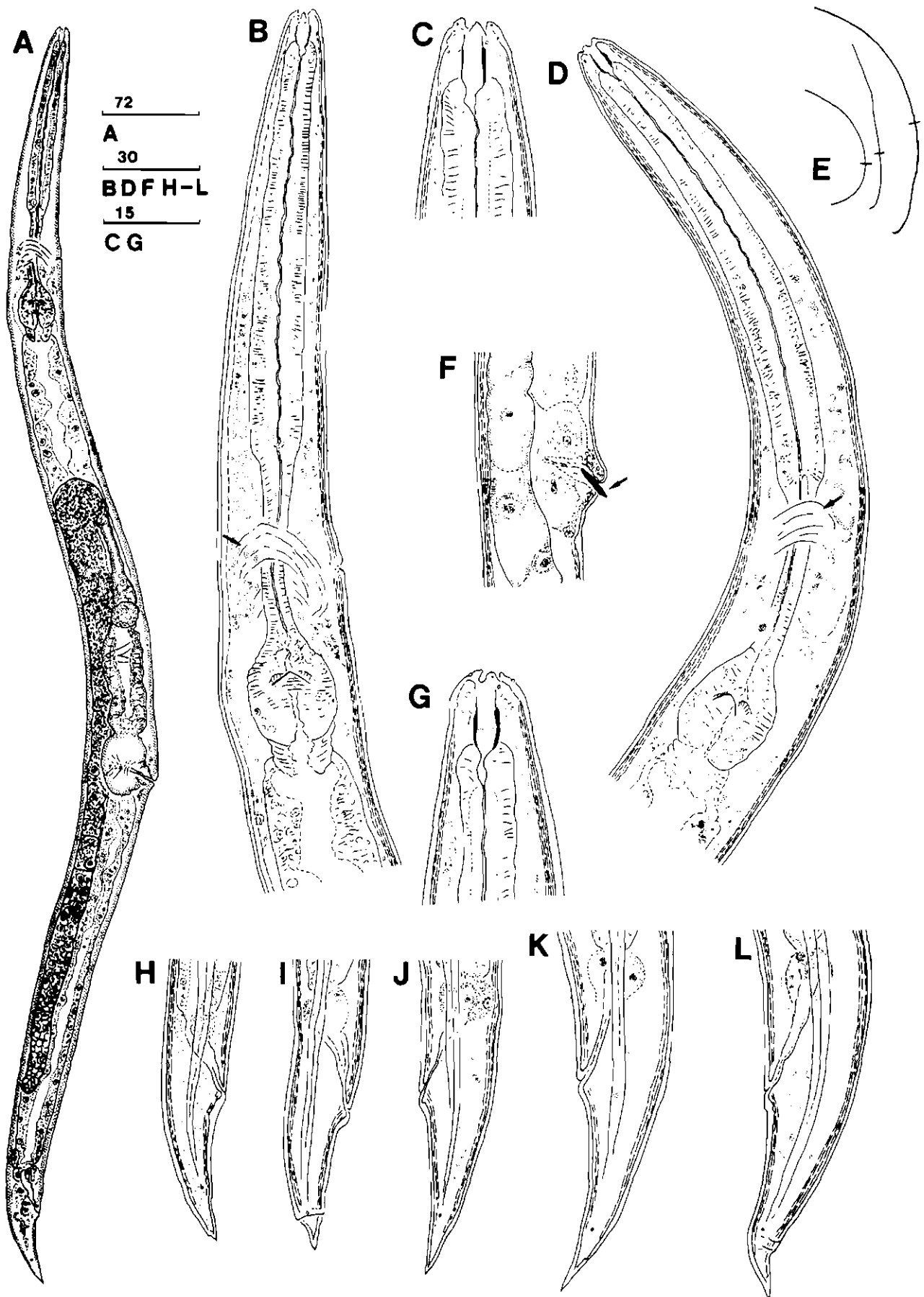
Figure 2 Panagrolaimus magnivulvatus Boström, 1995. Female. A-F & H-I. Population from algal mats. A: Entire body. B & D: Anterior region showing different positions of nerve ring (arrow) in two specimens. C: Head end. E: Heat-relaxed body posture. F: Vulval region showing refractive object protruding from vulva. H-I: Tails of different specimens, showing bifurcated tail tip (H) and retracted tail tip (I). G & K-L. Population from nest material. G: Head end. K-L: Tails of different specimens.
