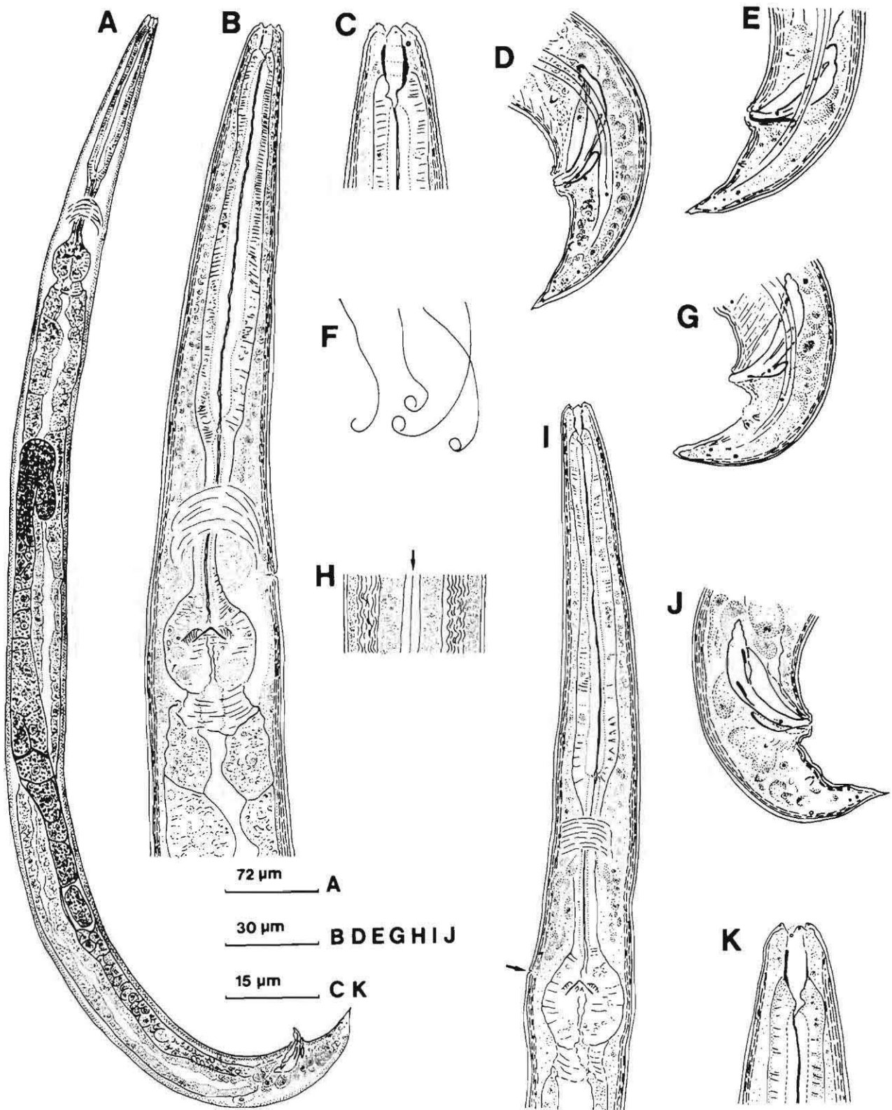
Figure 3 Panagrolaimus magnivulvatus Boström, 1995. Male. A–H: Population from algal mats. A: Entire body. B: Anterior region. C: Head end. D–G: Tails showing bifurcated tail tip (E) and aberrant male with atypical tail tip and arrangement of caudal papillae (G). F: Heat-relaxed body posture. H: Three lateral incisures (arrow) in lateral field. I–K: Population from nest material. I: Anterior region showing excretory pore located in a very posterior position (arrow). J: Tail. K: Head end.
