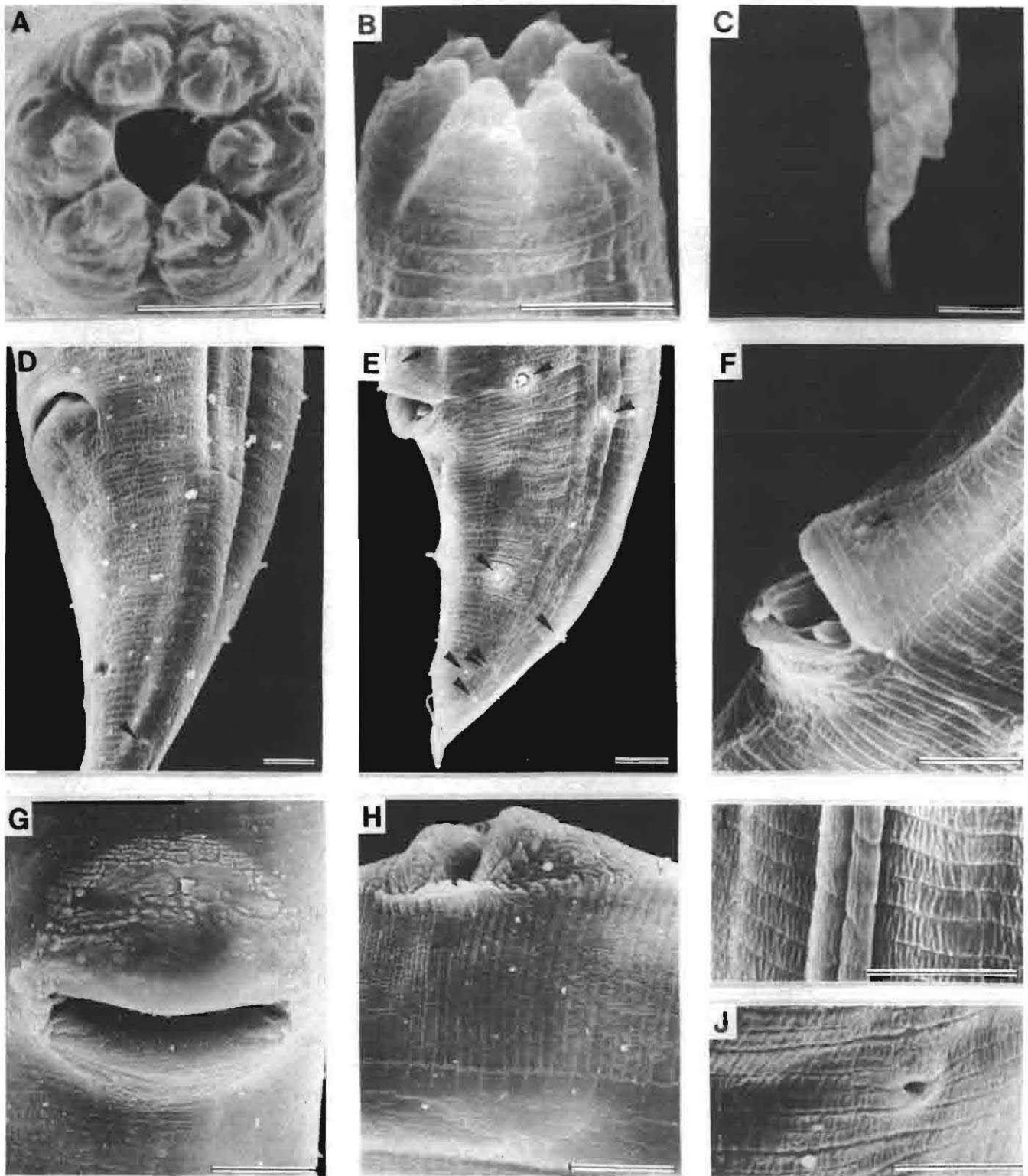
Figure 4 Panagrolaimus magnivulvatus Boström, 1995. Population from algal mats. A: Female head in frontal view. B: Female head in ventro-lateral view. C: Bifurcated tail tip (female). D: Anal region of female showing phasmid (arrow). E: Male tail showing caudal pores (single arrow) and phasmid (double arrow). F: Cloacal opening showing adanal papilla (arrow). G: Vulva in ventral view. H: Vulva in lateral view. I: Lateral incisures in female in midbody region. J: Excretory pore in male. Bar equals 5 \mu\text{m} in all photomicrographs except in C where bar equals 1 \mu\text{m} .
