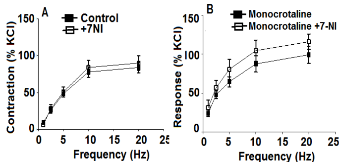
Fig. 4 Effect of 7NI, ( 10^{-4} M), a selective inhibitor of inducible nitric oxide synthase, on EFS-induced contractions of pulmonary artery ring segments isolated from control (A) and monocrotaline-treated pulmonary hypertensive rats (B). ■ and □ represent EFS-induced contractions in the absence and in the presence of 7NI, respectively. Each point on the graph is the mean \pm S.E.M of 4 (monocrotaline-treated rats) and 6 (control rats) experiments.
