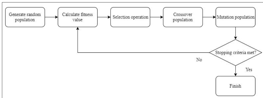
Fig.2. Basic Operation of Genetic Algorithm
