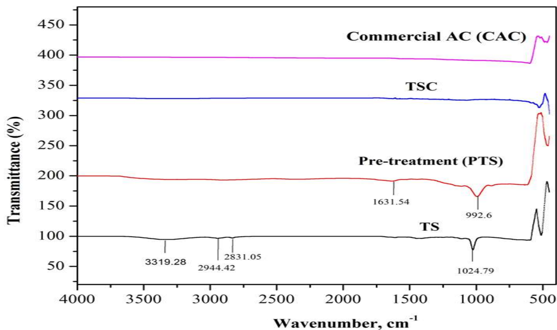
Fig.2. FTIR spectra of commercial AC (CAC), TSC, PTS and TS
