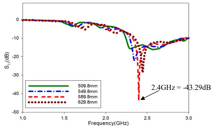
Fig.3. The effects on reflection coefficient, S_{11} due to change of length monopole plasma antenna.
