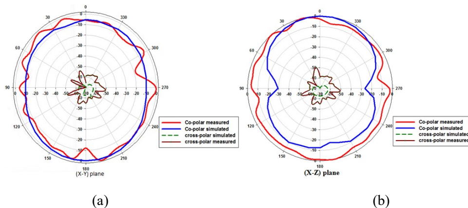
Fig.6. Simulated and measured radiation patterns of monopole plasma antenna (ON) at 2.4 GHz in (a) H-Plane and (b) E-Plane.
