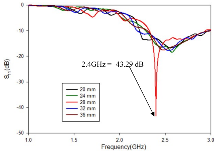
Fig.4. The effects on reflection coefficient, S_{11} due to change of the diameter of plasma antenna.
