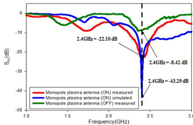
Fig.5. Simulated and measured reflection coefficient, S_{11} for monopole plasma antenna.
