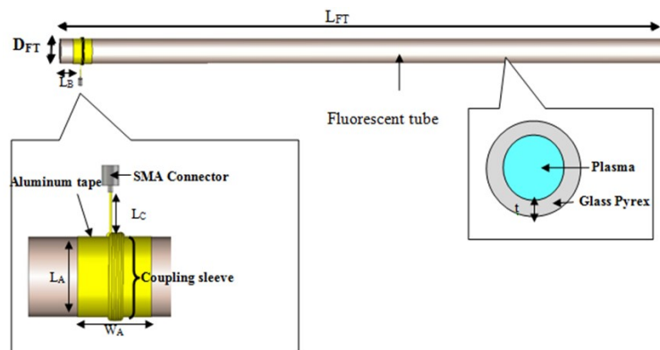
Fig.1. The structure of a monopole plasma antenna.
