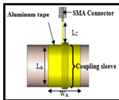
Fig. 2. Coupling sleeve structure.
