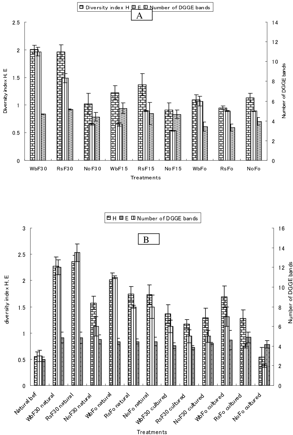
Fig. 2. Shannon's diversity index ( H ), equitability ( E ), and number of DGGE bands of bacterial 16S rDNA from greenhouse ( A ) and field ( B ) samples. Wb: wheat bran; Rs: rice straw; No: no organic matter; F0, F15, and F30: no flooding, 15-day flooding, and 30-day flooding, respectively. In ( B ), bacterial 16S rDNA was extracted from two types of sclerotia: sclerotia from Sclerotium rolfsii cultured on PDA (cultured sclerotia) or sclerotia from greenhouse-grown diseased plants (natural sclerotia). The sclerotia were buried in soil with or without 30-day flooding. "Natural" and "cultured" refer to bacterial 16S rDNA samples from natural and cultured sclerotia, respectively; "natural bef" refers to samples from natural sclerotia before burial in the soil.
