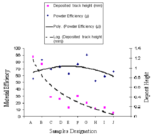
Figure 6: Variation of the material efficiency and the deposit height against the scanning speed
