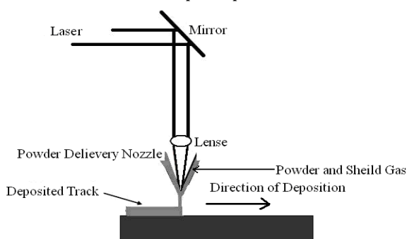
Figure 1: Schematics of Laser Metal Deposition Process
