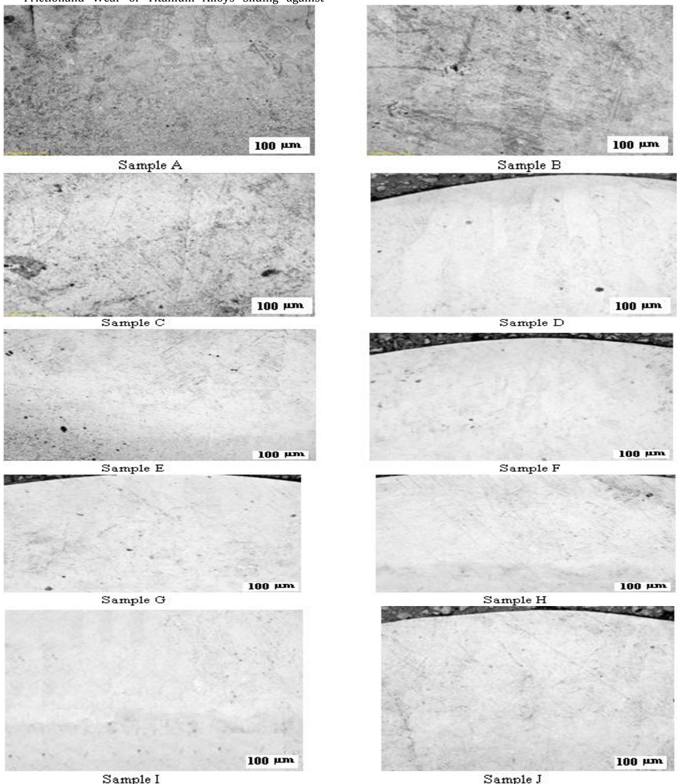
Figure 7: The macrostructure of the samples A to J showing the deposit layer and the substrate
