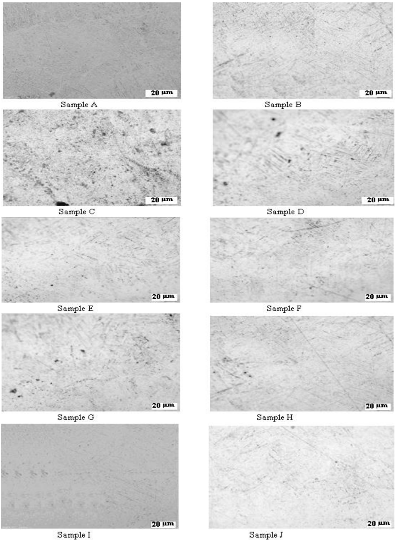
Figure 8: The microstructure of the samples A to J showing the fusion zone between the deposit and the substrate
