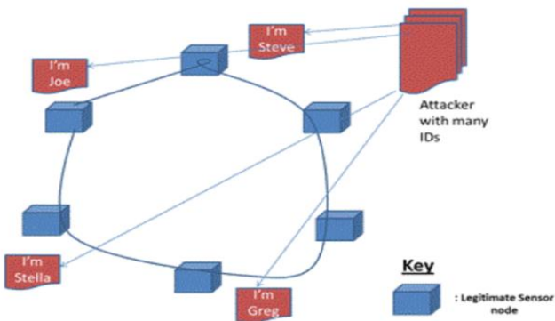
Figure 2: Sybil Attack [4].
