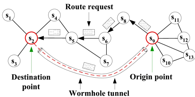
Figure 5: Wormhole Attack [14]
