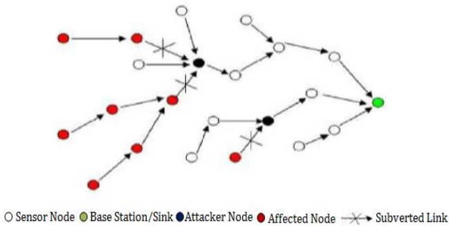
Figure 3: Blackhole Attack [8]
