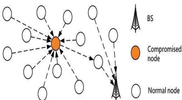
Figure 6: Sinkhole Attack [14]
