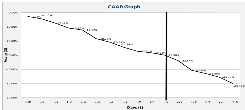
Figure 3: Graphical representation of CAAR for the 16-day event window
