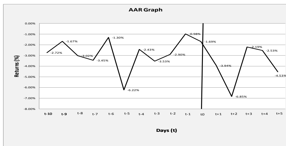
Figure 2: Graphical representation of AAR for the 16-day event window
