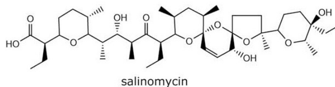
Figure 1. Structure of salinomycin.
