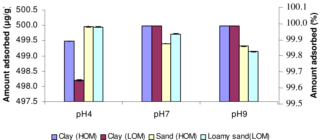
Figure 5. Effect of pH on adsorption of salinomycin at 500 µg/g soil.
