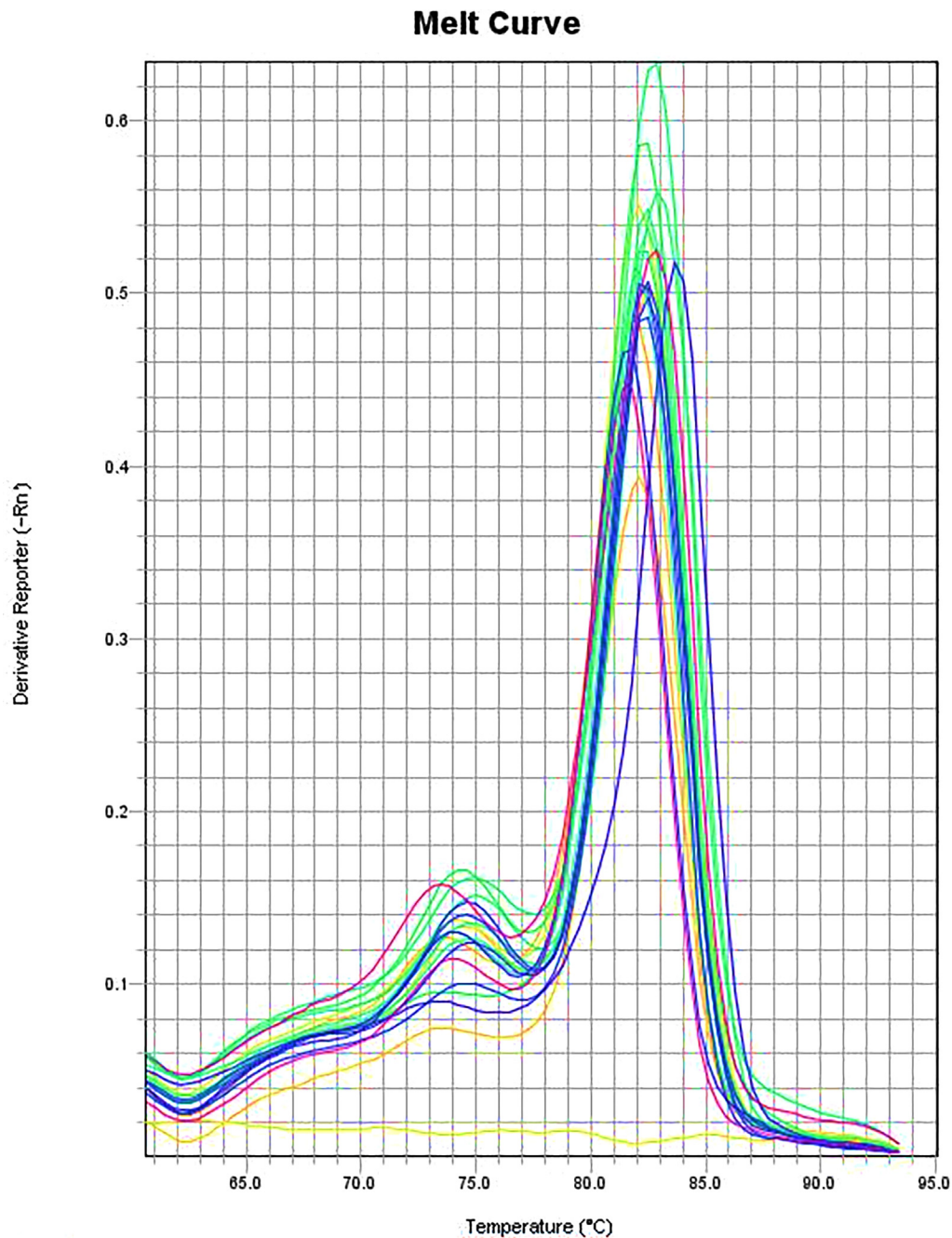
Fig. 2. Melting curve identifying specificity of chosen primers.
