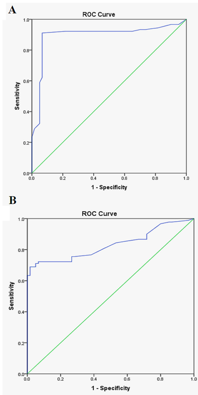
Fig. 4. a. ROC curve of serum AFP levels for diagnosis of HCC, b. MTDH mRNA expression level for diagnosis of HCC.
