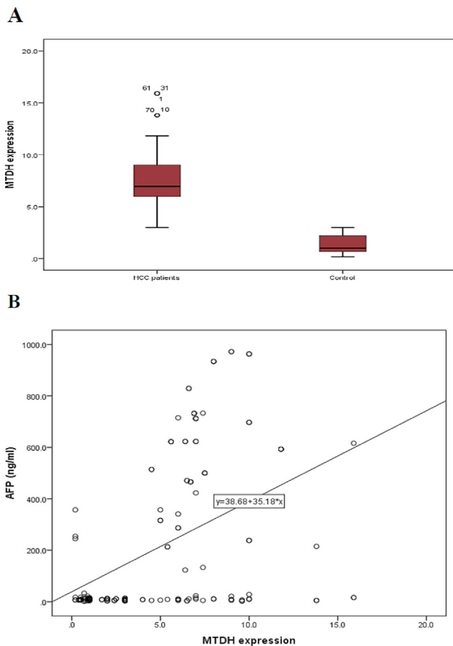
Fig. 3. a. Expression level of MTDH mRNA in studied groups, b. Correlation between MTDH mRNA relative expression & serum AFP levels in HCC patients (r = 0.823), P value = <0.05.
