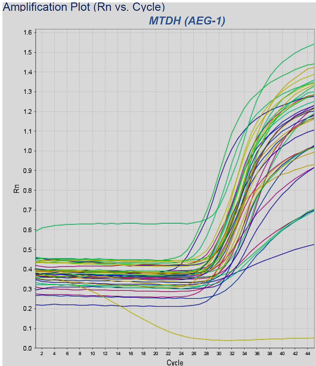
Fig. 1. Amplification plot of MTDH expression (normalized fluorescence signal (Rn) plotted versus cycle number).
