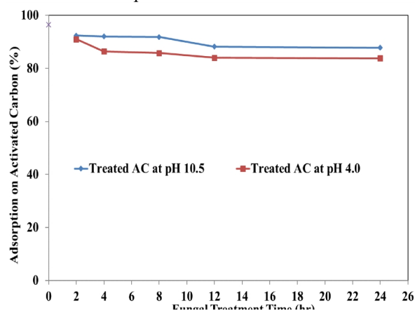
Fig. 2 Percentage Au Adsorption against Fungal Treatment Time at pH 4.0 and 10.5
