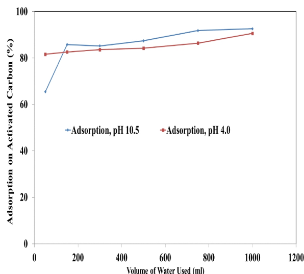
Fig. 3 Gold Adsorption against Volume of Water Used at pH 4.0 and 10.5
