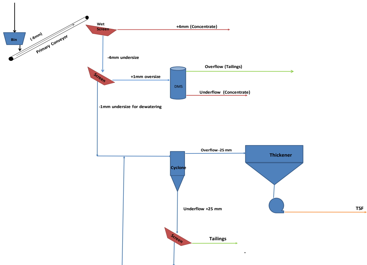
Fig. 3 Conceptual Flow Diagrams for the Fines Upgrade
