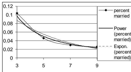
cousin marriage probability estimates (rates per available) fit to small world searchability power law 1/d^\alpha , d =distance and \alpha=1.6 power
