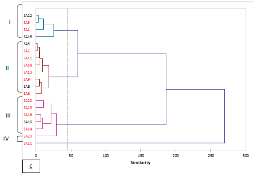
Figure 2: Dendrogram showing diversity within rock phosphate solubilizing isolates (in red color) obtained from soil samples collected at Nkobisson (a, similarity < 300%), Nyokon (b, similarity < 100%) and Santchou (c, similarity < 50%). Isolates are distributed into four main groups numbered I, II, III, IV.
