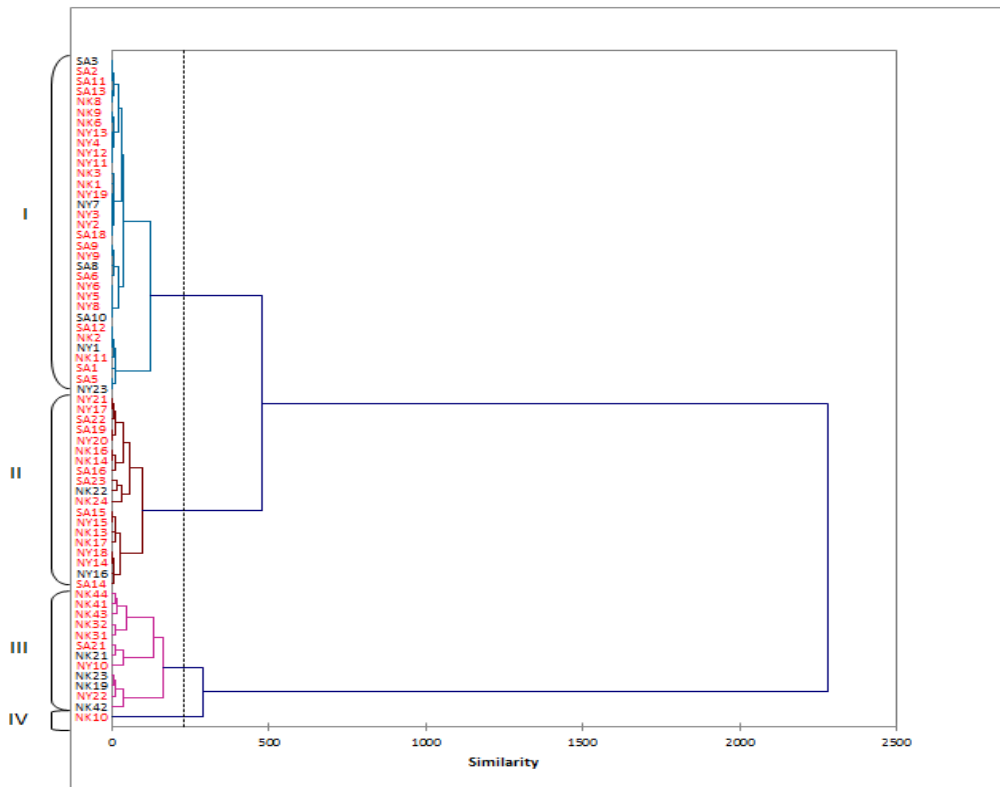
Figure 3: Dendrogram showing cumulative diversity within rock phosphate solubilizing isolates (in red color) obtained from soil samples collected at the three sampling sites (similarity < 250%). Isolates are distributed into four main groups numbered I, II, III, IV.
