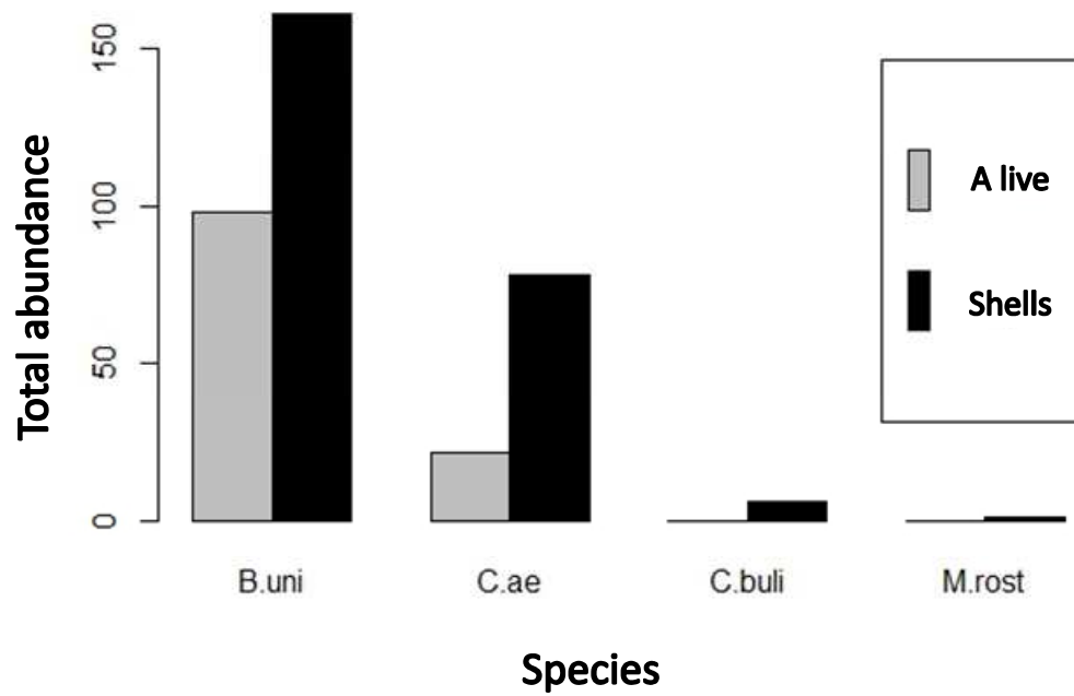
Figure 5: Total abundance of living specimens and empty shells. B.uni: Bellamya unicolor , C.aeg: Coelatura aegyptiaca , Cl.bul: Cleopatra bulimoïdes , M.rost: Mutela rostrata .
