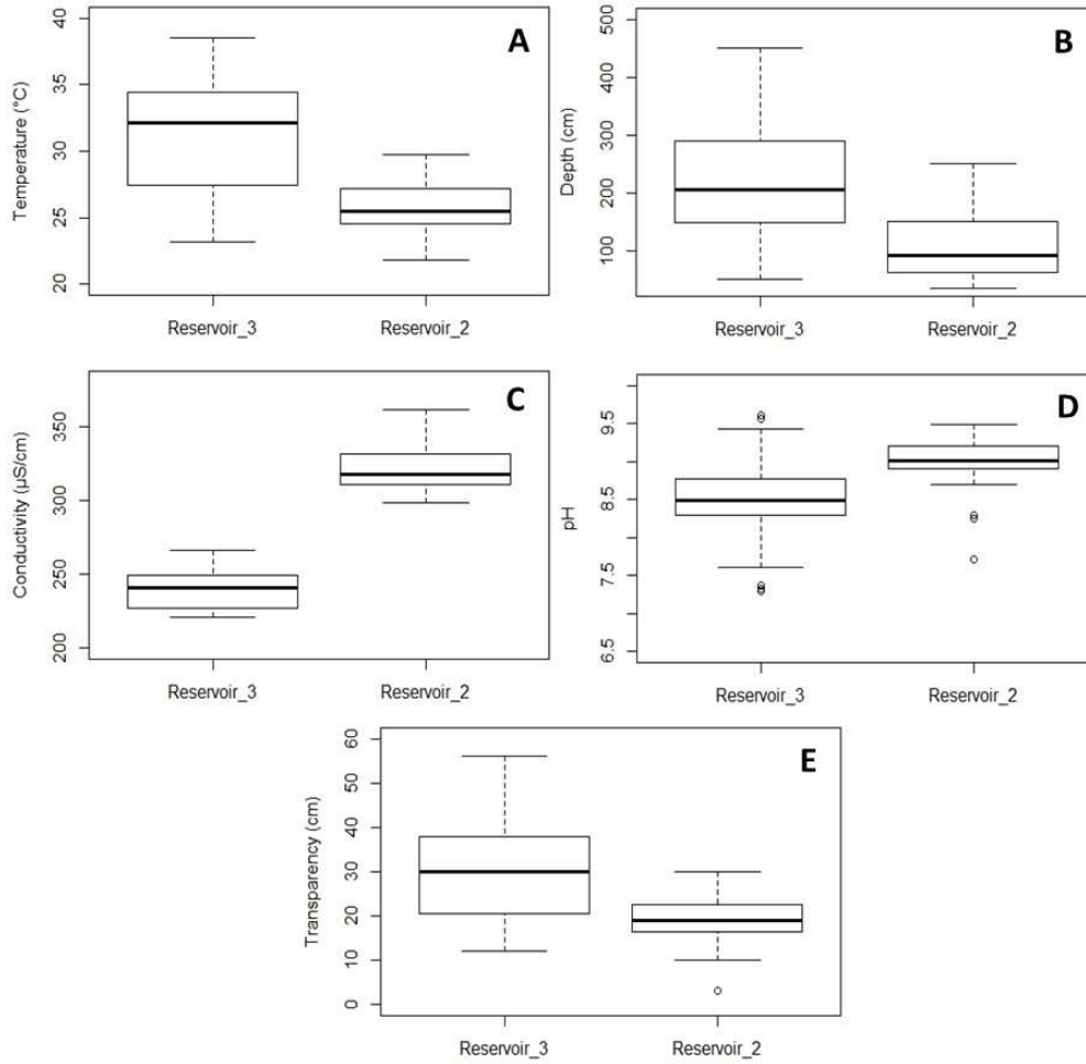
Figure 2: Boxplot showing physicochemical variables distribution in the two reservoirs. A= temperature (°C); B= Depth (cm); C= Conductivity (µS/cm); D= pH; E= Transparency (cm).
