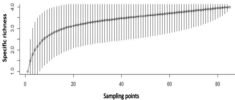
Figure 3: Rarefaction curve in relation to sampling points in the studied reservoirs.
