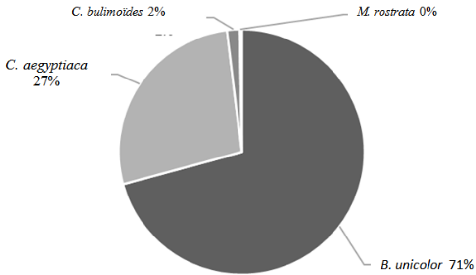
Figure 4: Species proportion in the reservoirs (n°2 and n°3) of Ouagadougou.
