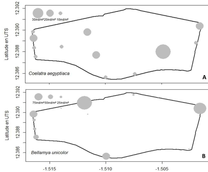
Figure 6: Spatial distribution of C. aegyptiaca and B. unicolor in the reservoir n°3 of Ouagadougou. A= Spatial distribution of C. aegyptiaca ; B= Spatial distribution of B. unicolor .
