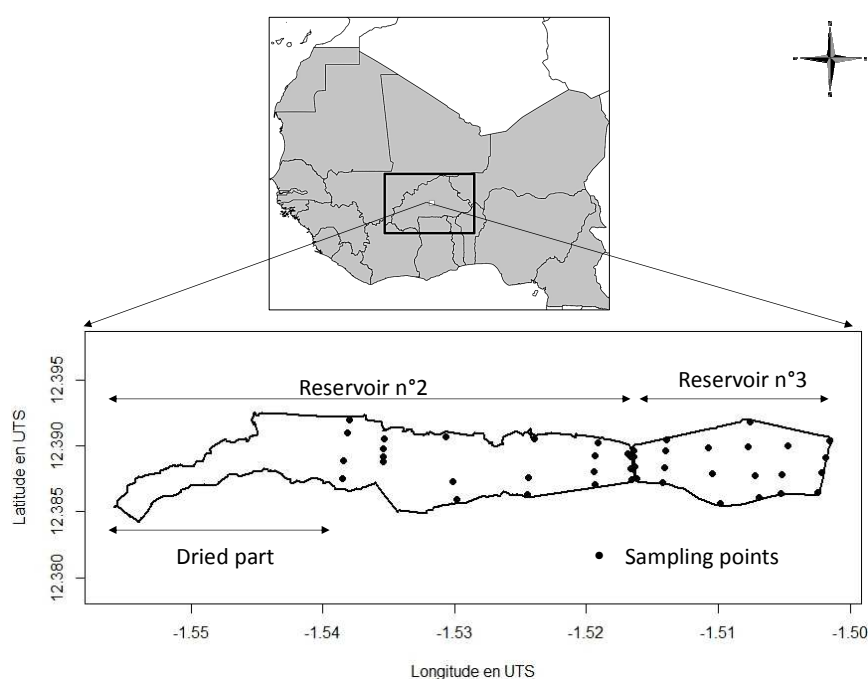
Figure 1: Presentation of study area and sampling design.
