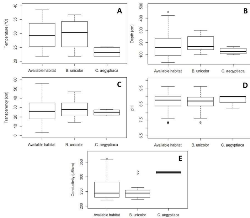
Figure 7: Habitats used by C. aegyptiaca and B. unicolor in the reservoir n°3 of Ouagadougou. A= Habit use by B. unicolor and C. aegyptiaca following water temperature; B= Habit use by B. unicolor and C. aegyptiaca following water column depth; C= Habit use by B. unicolor and C. aegyptiaca following water Transparency; D= Habit use by B. unicolor and C. aegyptiaca following water pH; E= Habit use by B. unicolor and C. aegyptiaca following water conductivity.
