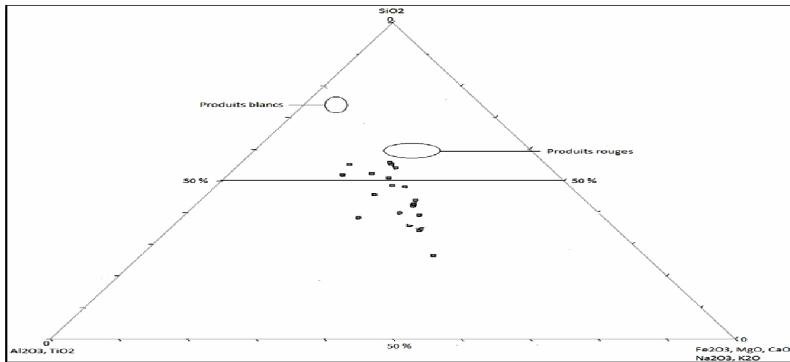
Figure 8 : Diagramme ternaire \text{SiO}_2/\text{Al}_2\text{O}_3 , \text{TiO}_2/\text{Fe}_2\text{O}_3 , \text{MgO} , \text{CaO} , \text{Na}_2\text{O}_3 , \text{K}_2\text{O}
