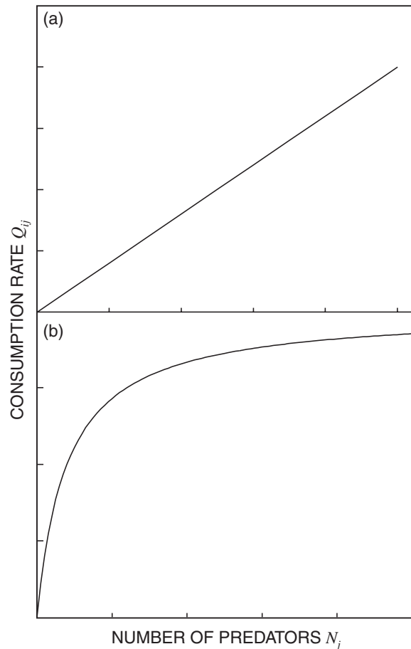
Fig. 1: Schematic showing how the total consumption rate Q_{ij} of prey species i by predator species j grows as the number of predators increase for the two contrasted cases – (a) MSVPA (and its derivatives providing projections) showing a linear proportionality relationship, (b) ECOSIM’s foraging arena-based model in which the total rate saturates at a constant level for high numbers of predators
