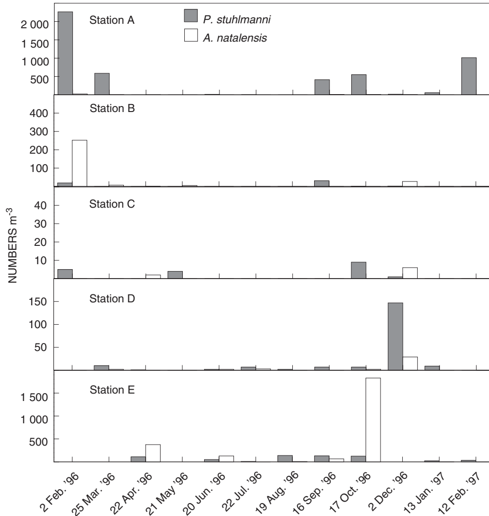
Fig. 5: Monthly abundance of Pseudodiaptomus stuhlmanni and Acartia natalensis sampled at Stations A–E between 1996 and 1997
