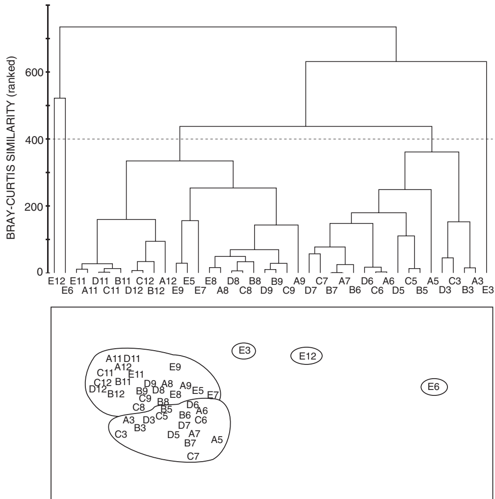
Fig. 6: Cluster analysis and corresponding multi-dimensional scaling (MDS) plot of zooplankton sampled at the five stations (A–E) in the Mhlathuze Estuary in 1996 and 1997. Only sampling periods where all five stations were sampled are included in the analysis. Numerals denote months, i.e. 3 = Apr '96, 5–9 = Jun '96–Oct '96, 11,12 = Jan '97, Feb '97. Codes on the MDS plot that overlap were moved adjacent to each other for clarity, without affecting the groupings
