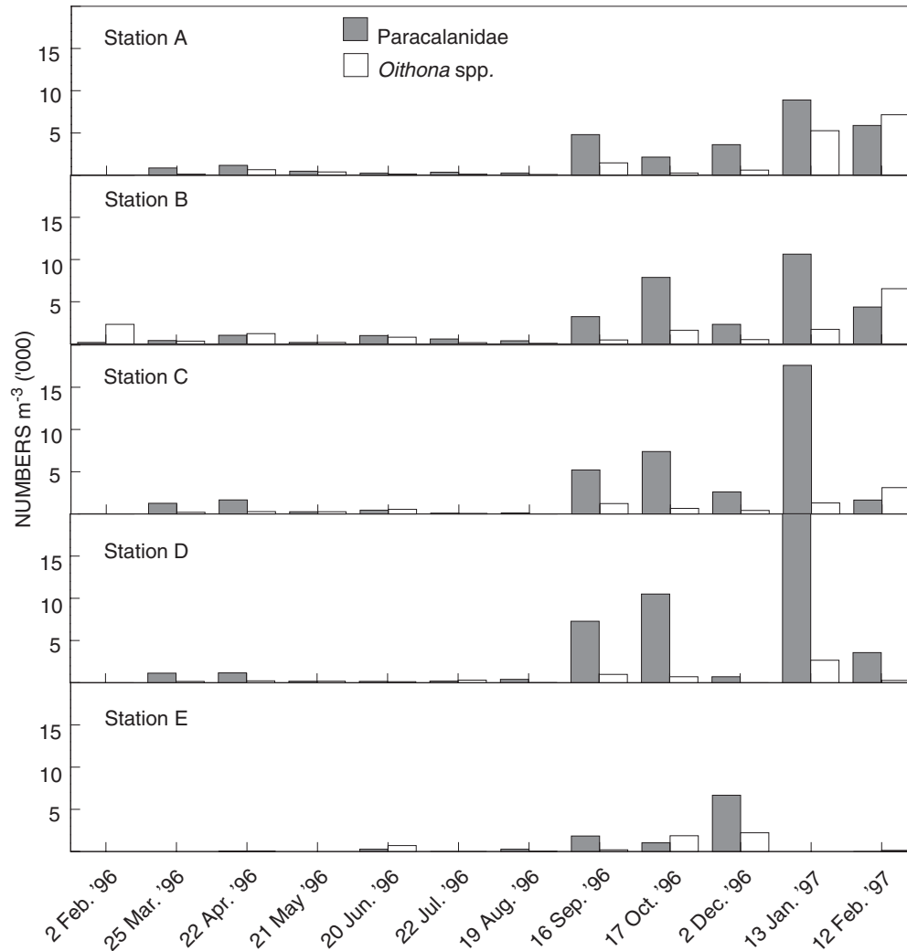
Fig. 4: Monthly abundance of Paracalanidae and Oithona spp. sampled at Stations A–E between 1996 and 1997
