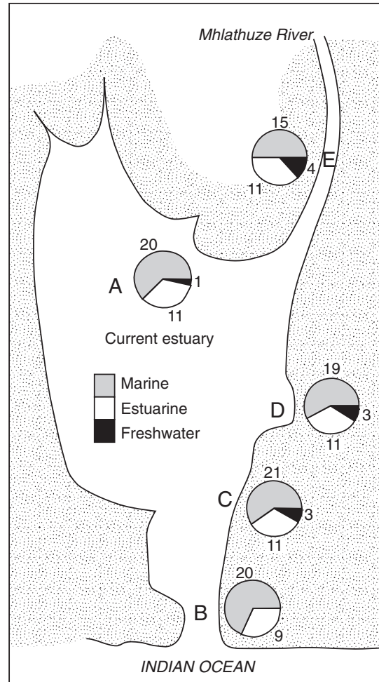
Fig. 3: Total number of marine, estuarine and freshwater taxa sampled at Stations A–E between 1996 and 1997
