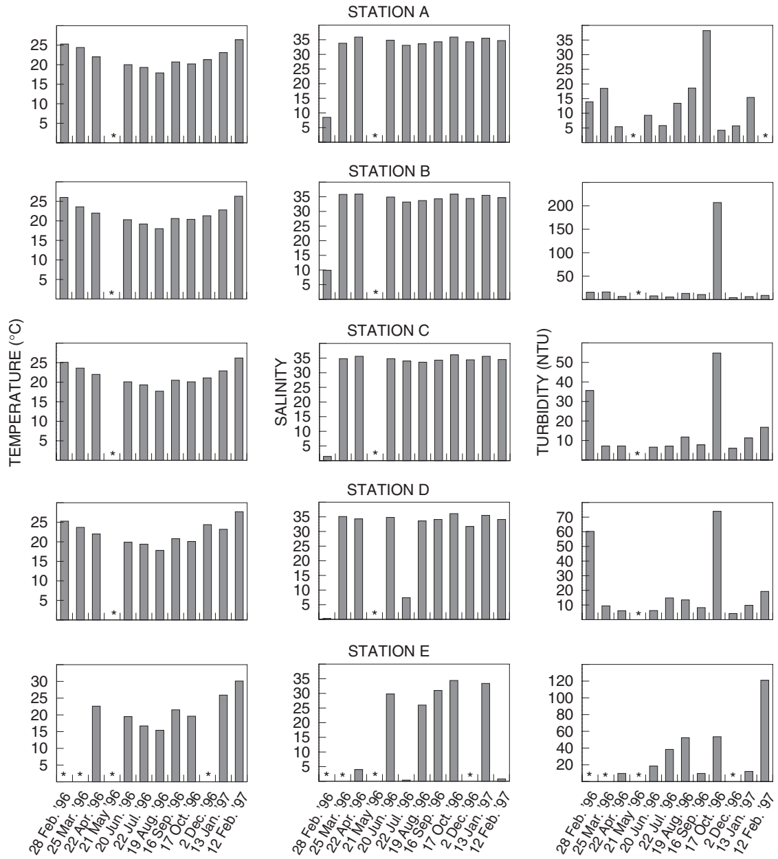
Fig. 2 Trends in temperature, salinity and turbidity at Stations A–E, 1996–1997. Note that no measurements were taken in May 1996 as a result of instrument failure
