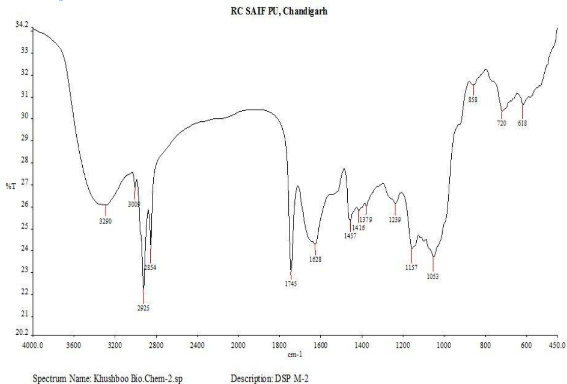
Figure 7: FT-IR spectra of methanolic extract of Datura metel seeds
