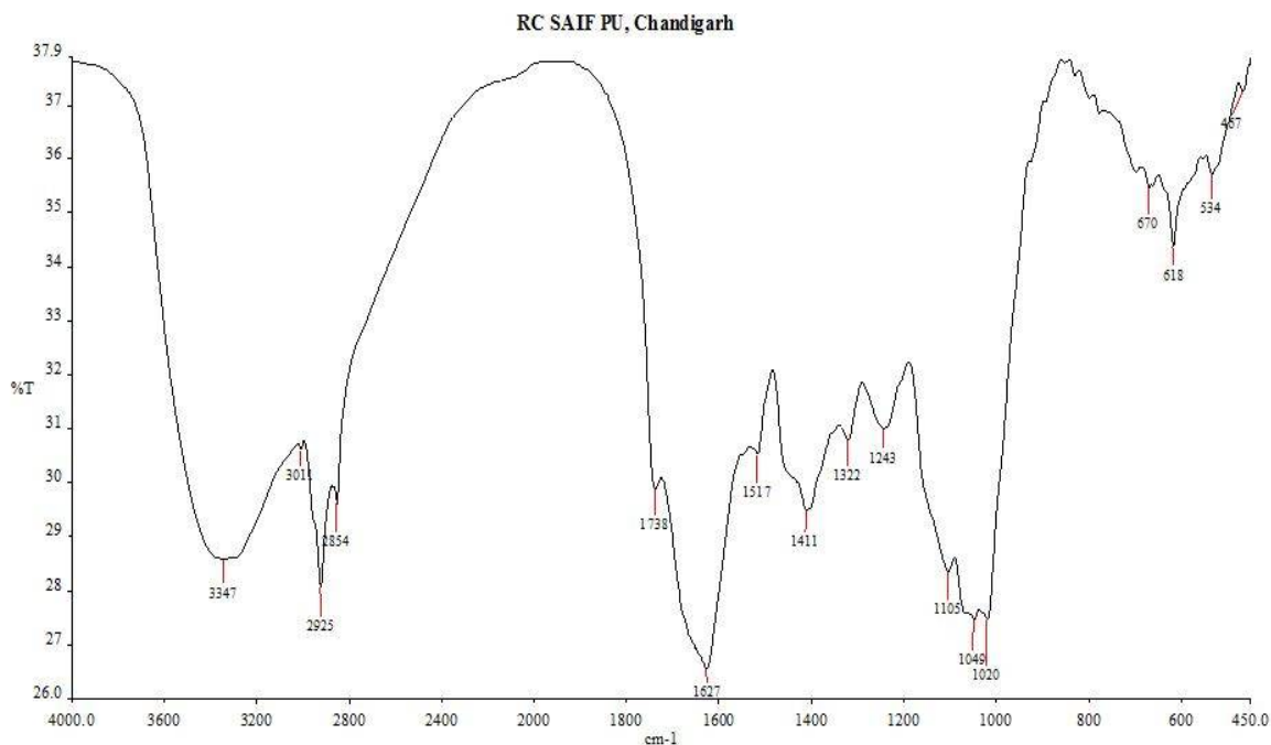
Figure 4: FT-IR spectra of methanolic extract of Datura innoxia leaves
