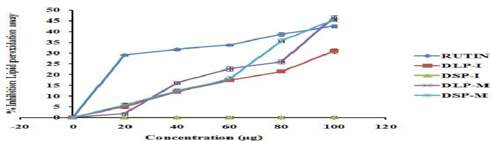
Figure 3: Lipid peroxidation inhibition activity of Datura innoxia and Datura metel leaf & seed methanolic extracts. Values are represented as mean \pm SD (n = 3). DLP-I ( Datura innoxia leaf extract), DSP-I ( Datura innoxia seeds extract), DLP-M ( Datura metel leaf extract), DSP-M ( Datura metel seeds extract).
