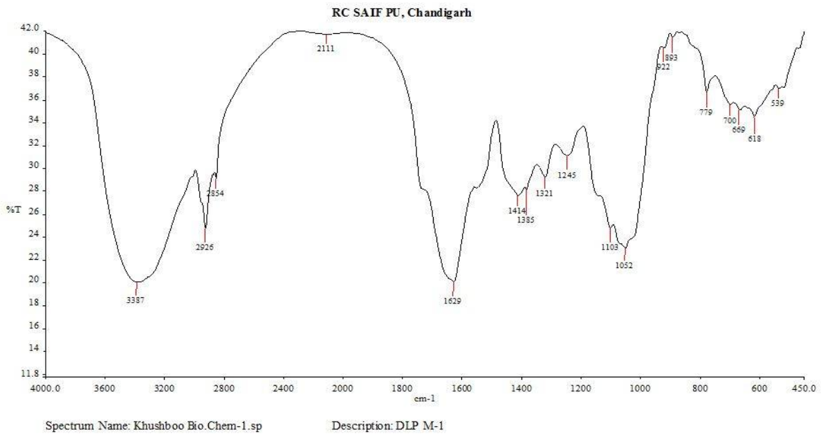
Figure 6: FT-IR spectra of methanolic extract of Datura metel leaves
