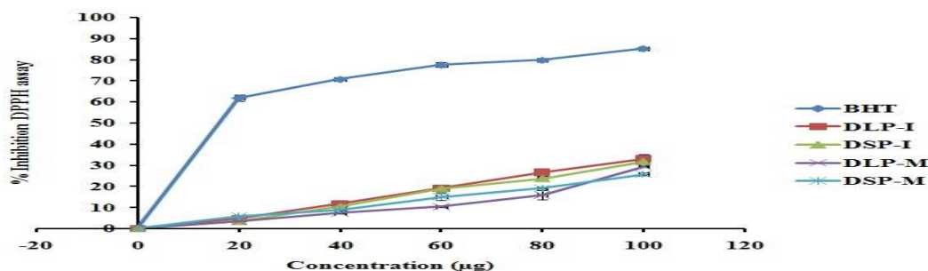
Figure 1: DPPH radical scavenging activity of Datura innoxia and Datura metel leaf & seed methanolic extracts. Values are represented as mean \pm SD (n = 3). DLP-I ( Datura innoxia leaf extract), DSP-I ( Datura innoxia seeds extract), DLP-M ( Datura metel leaf extract), DSP-M ( Datura metel seeds extract).
