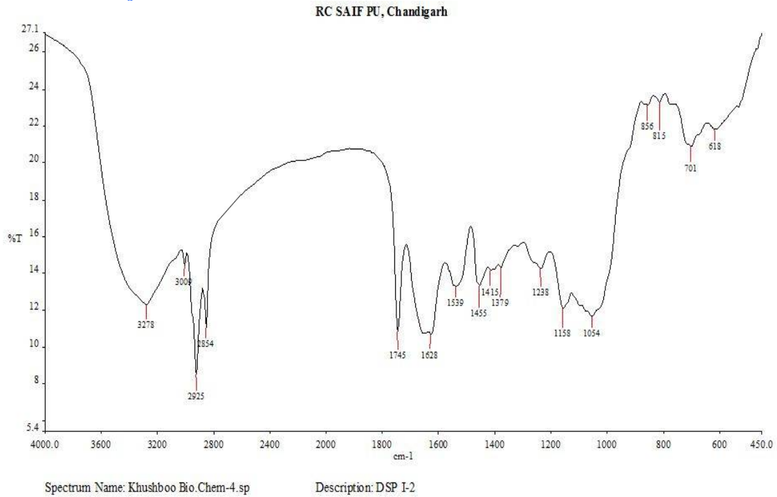
Figure 5: FT-IR spectra of methanolic extract of Datura innoxia seeds
