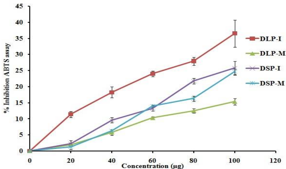
Figure 2: ABTS radical cation scavenging activity of Datura innoxia and Datura metel leaf & seed methanolic extracts. Values are represented as mean \pm SD (n = 3). DLP-I ( Datura innoxia leaf extract), DSP-I ( Datura innoxia seeds extract), DLP-M ( Datura metel leaf extract), DSP-M ( Datura metel seeds extract).
