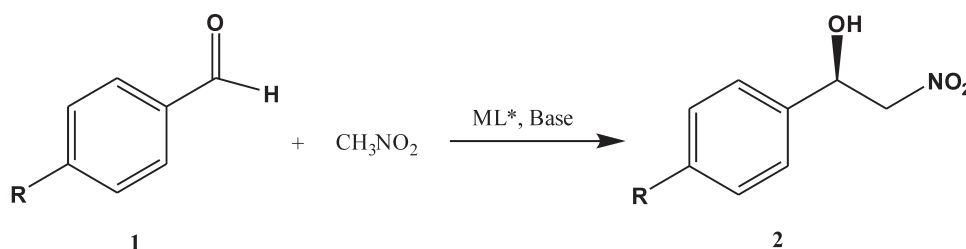
Scheme 1 The asymmetric Henry reaction.
