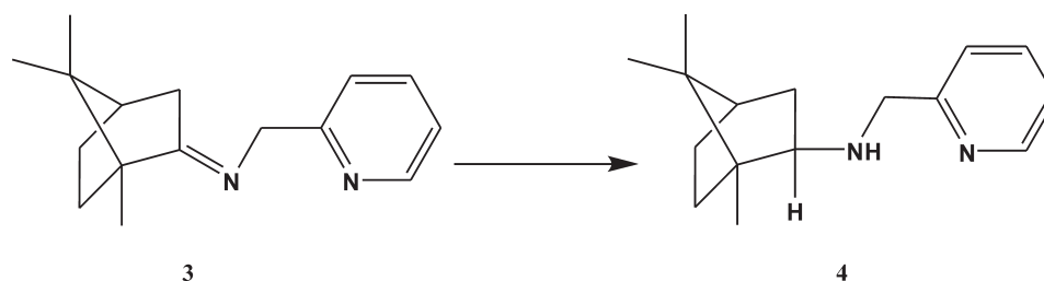
Scheme 2 Example of a previously successful camphor-derived ligand 7 .
