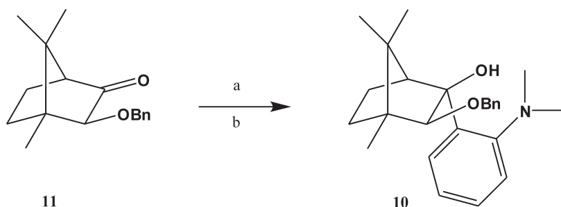
Scheme 4 Synthesis of Ligand 10. Key: (a) 11, \text{CeCl}_3 , RT, 30 min; (b) 2-(dimethylamino)phenyllithium, -78\text{ }^\circ\text{C} \rightarrow \text{RT} , 12 h.
