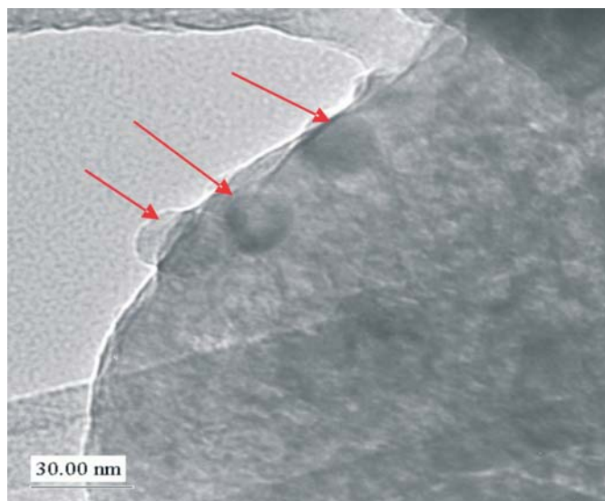
Figure 3 TEM image of IMPN. Arrows show some Fe-Co nanoparticles (~30 nm) supported on \text{CaCO}_3 after calcination.
