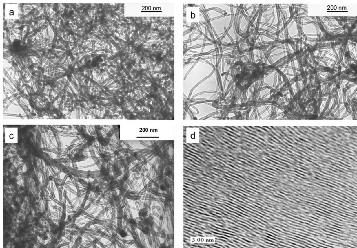
Figure 4 TEM images of MWCNTs prepared by the (a) IMPN, (b) DPN, (c) RM methods and (d) a general higher magnification TEM image showing a much closer look at the 'wavy-like' 0.34 \text{ nm} (0002) graphite lattice fringes of the CNTs.
