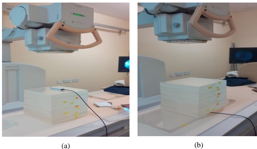
Figure 2: The experimental setup to measure (a) entrance surface air kerma and (b) image intensifier input kerma rates using Perspex slab phantom.
