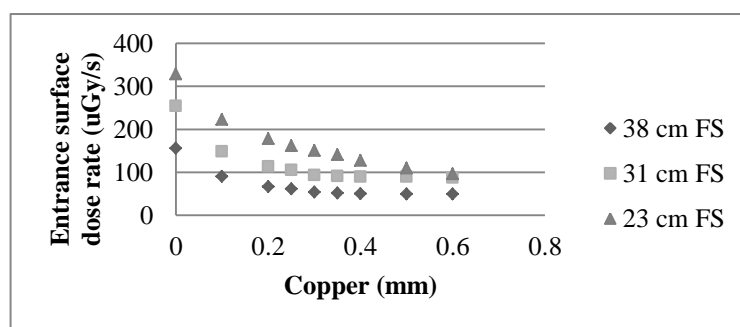
Figure 4: Entrance surface air kerma dose rate for fluoroscopic exposure of a 20 cm Perspex phantom for 38, 31, and 23 cm field size.
