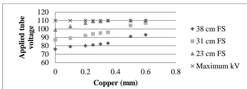
Figure 5: Automatic kV selection for fluoroscopic exposure of 20 cm Perspex phantom for 38, 31 and 23 cm field size.
