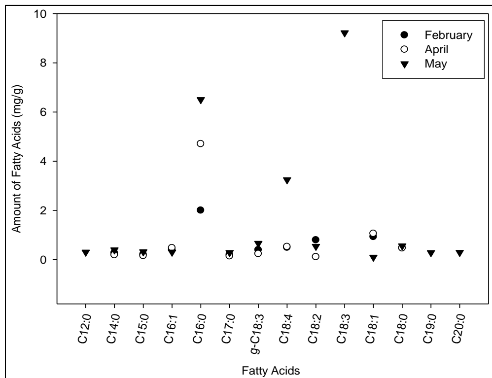
Figure 3: The variation of individual fatty acids in algae biomass samples collected between February and May 2013
