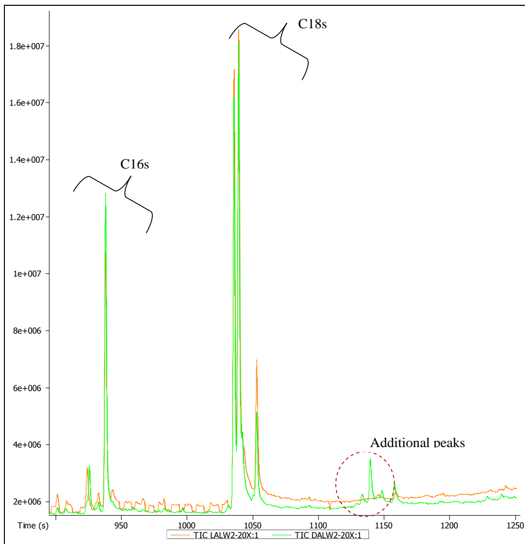
Figure 2: The overlaid GCxGC-TOFMS chromatograms for fatty acids from water filtrates from living and dead algal cells biomass showing the additional peaks of fatty acids on the water filtrate sample from dead algal cells (DALW; green coloured chromatogram) which were not observed on the water filtrate from the living algae cells biomass (LALW; brown coloured chromatogram).
