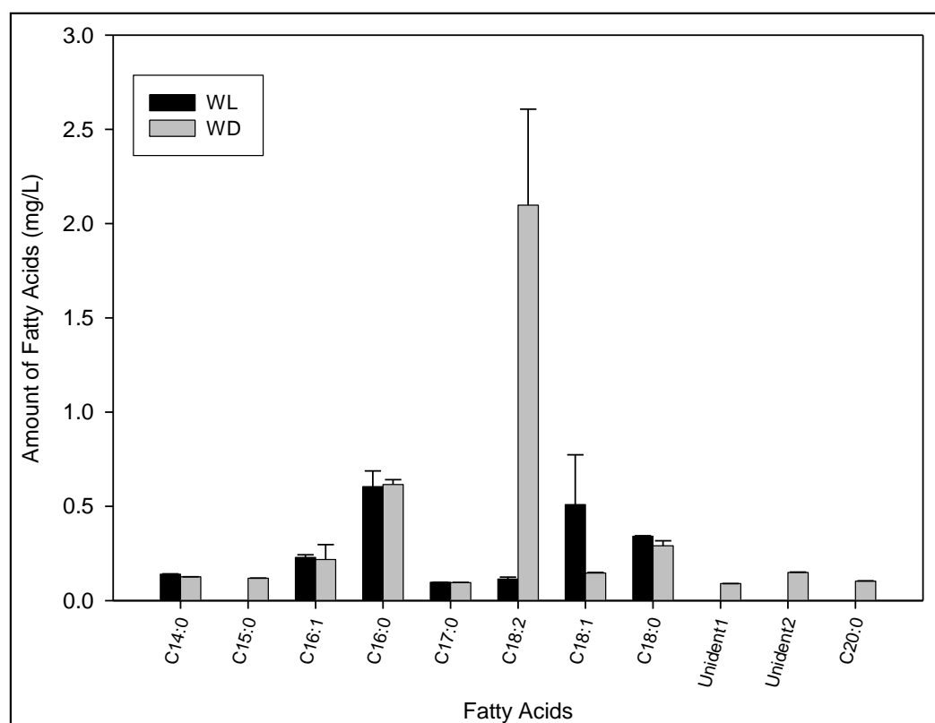
Figure 1: The variation of fatty acids in water samples from living (WL) and dead algal (WD) cells biomass (note; (Unident1 = Unidentified unsaturated fatty acid 1 and Unident2 = Unidentified unsaturated fatty acid 2)
