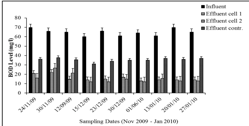
Figure 3: BOD levels (mg/L) in influent and effluents (cells 1, 2 and control) in the studied CW (Bars are standard deviation (+)).
