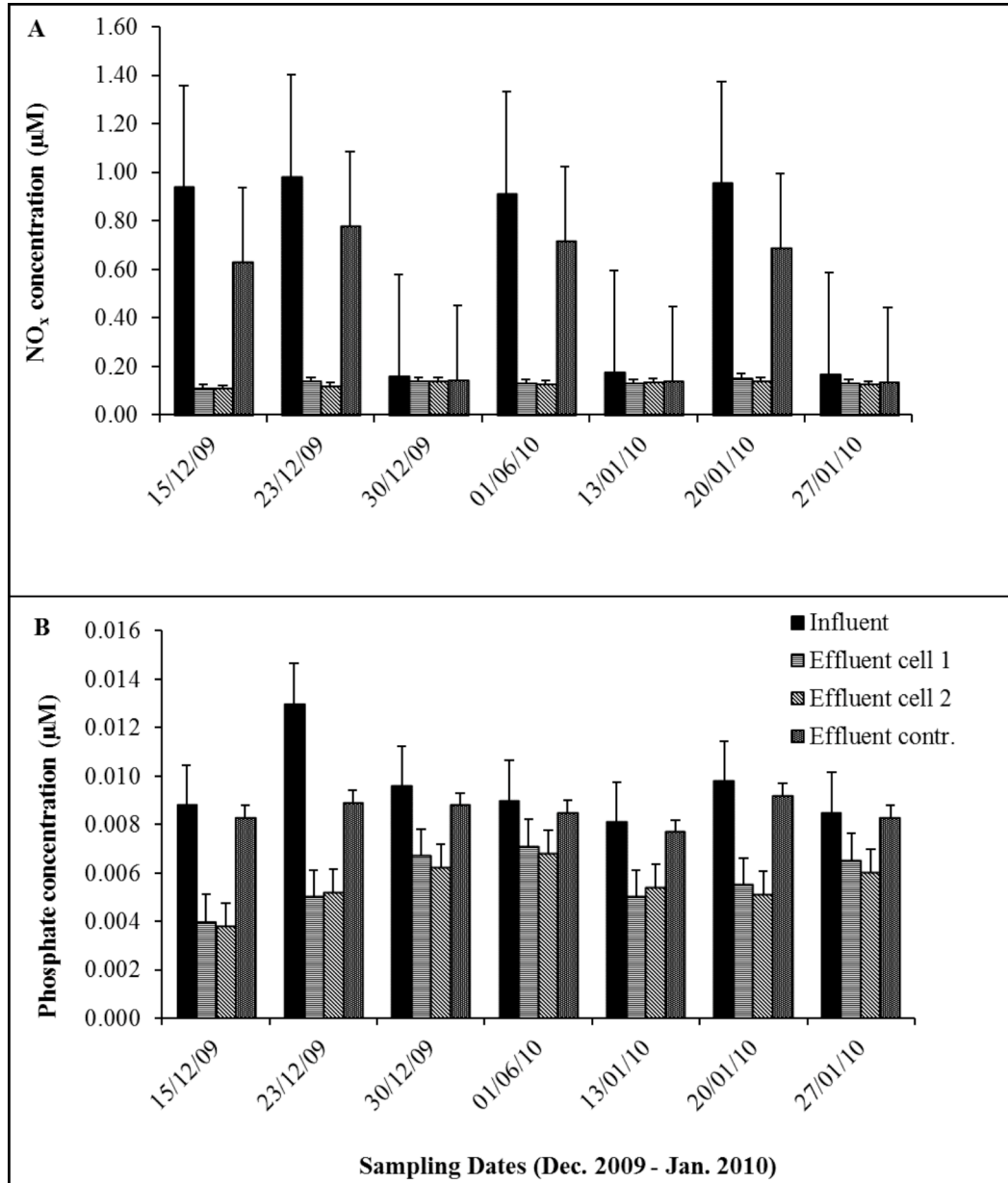
Figure 4: Average nutrient concentration during the different sampling occasions. A) Nitrate and nitrite combined (NO x ), (B) phosphate .
