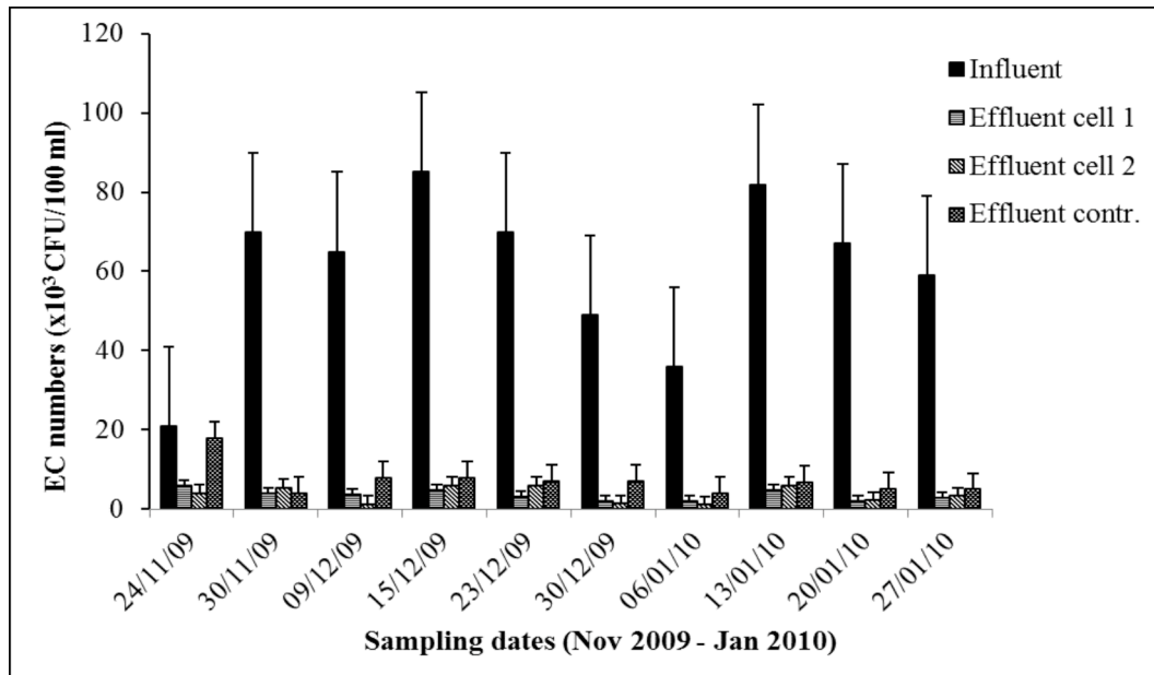
Figure 1: Mean concentration of E. coli in influents and effluents in cells 1, 2 and the control (Bars are standard deviation (+)).
