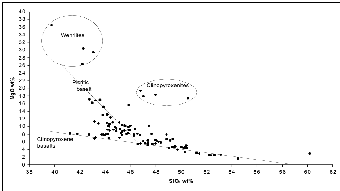
Figure 3 Variation plot of MgO wt% against SiO 2 wt% for the rocks from the Bufumbira volcanic field
