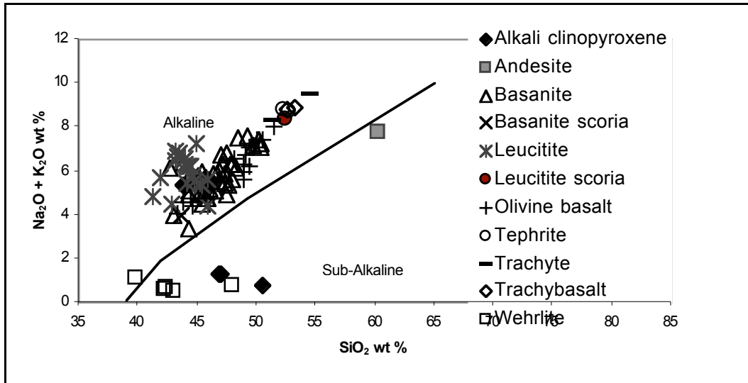
Figure 4: The plot of total alkalis ( \text{Na}_2\text{O} + \text{K}_2\text{O} wt%) versus \text{SiO}_2 wt% (after Irvine and Baragar 1971)
