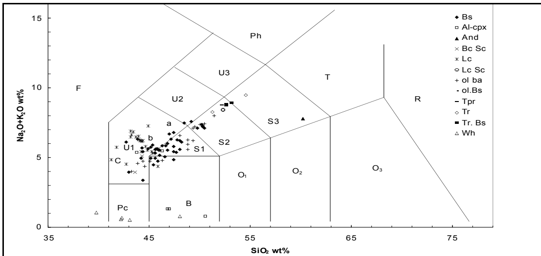
Figure 8 Diagram of total alkalis (Na 2 O + K 2 O wt%) against SiO 2 wt% of the Bufumbira basalts (after Le Maitre 1989)
