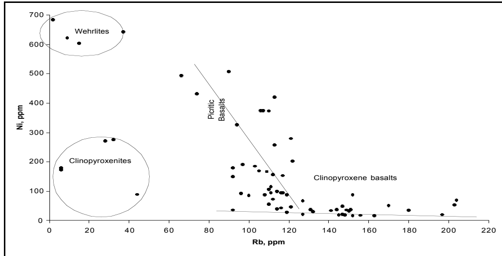
Figure 11: The binary diagram of Ni ppm versus Rb ppm
