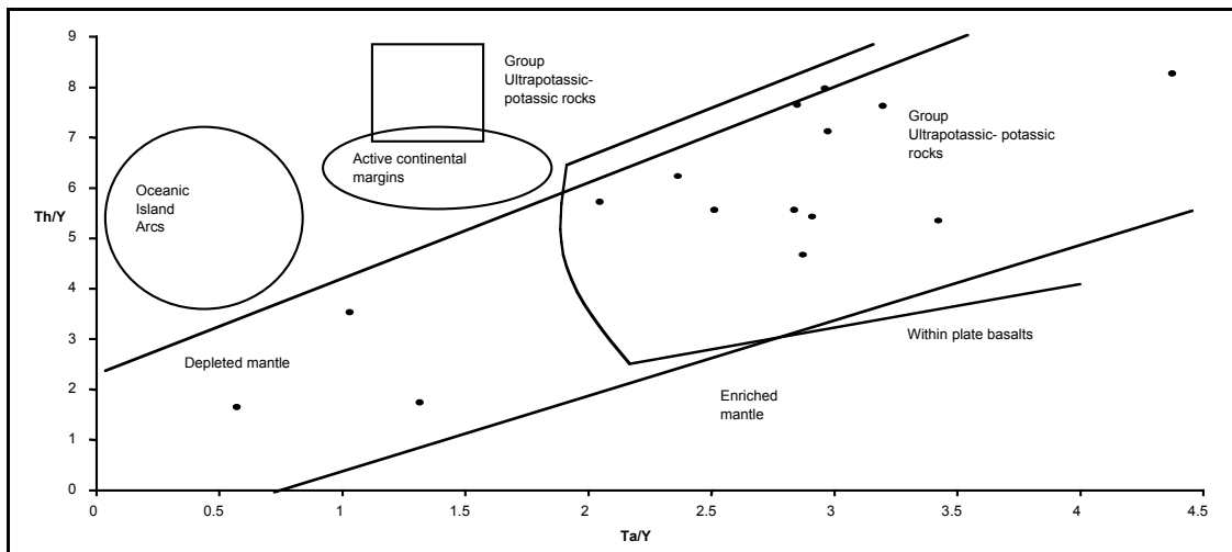
Figure 14: Plot of Th/Yb against Ta/Yb for samples of the Bufumbira volcanic rocks (after Pearce 1982, 1983)
