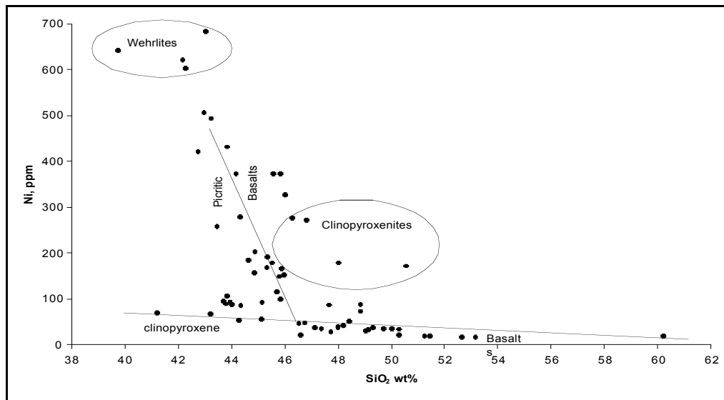
Figure 10 The variation plot of Ni ppm versus SiO 2 wt%
