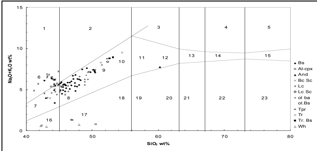
Figure 7: Variation diagram for total alkalis (Na 2 O + K 2 O wt%) against SiO 2 wt% (after Middlemost 1985)
