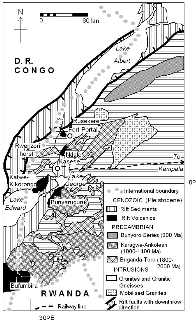
Figure 1 Geological map of Western Uganda (after Macdonald 1966) showing the small volcanic fields within the western branch of the East African rift system.
