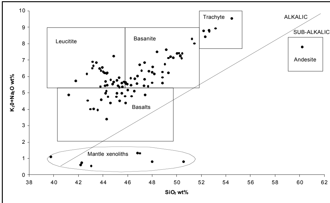
Figure 6: Plot of total alkalis ( K_2O + Na_2O wt%) versus SiO_2 wt% of the various rocks of the Bufumbira field (Cox et al. 1979)
