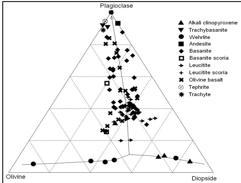
Figure 9 The Walker et al. (1989) normative ternary plot of plagioclase, olivine and diopside
