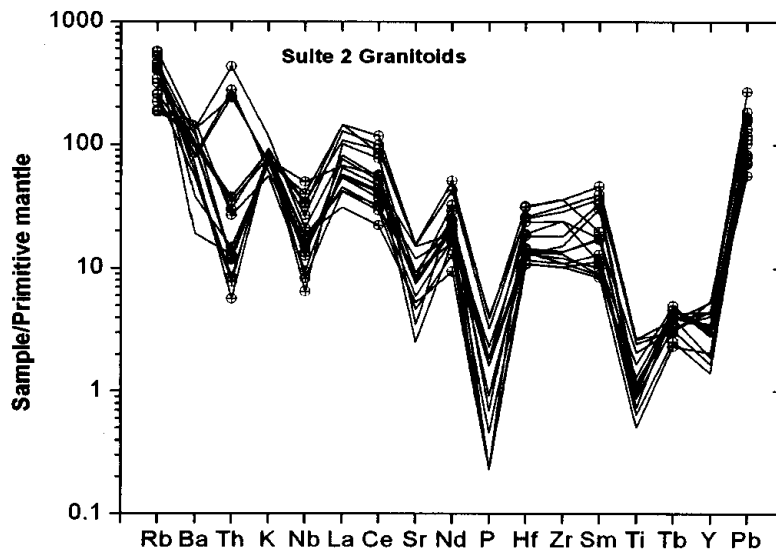
Figure 6: Primitive Mantle-normalised spidergrams for the Suite 2 granitoids.
