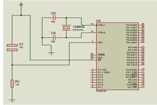
Fig 2: Microcontroller unit
