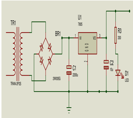
Fig. 1: The power supply unit
