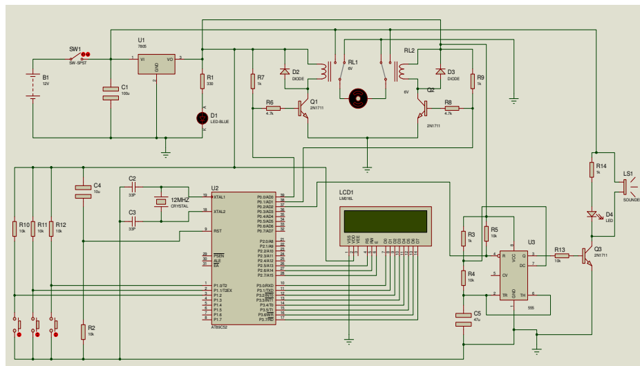
Fig 3: complete schematics diagram of an automatic fish feeder
