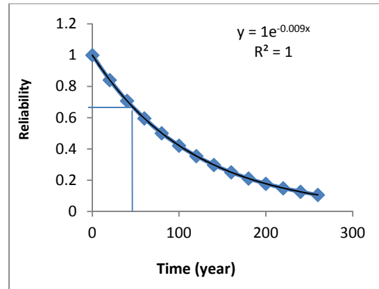
Fig 2: Reliability of Opon timber
