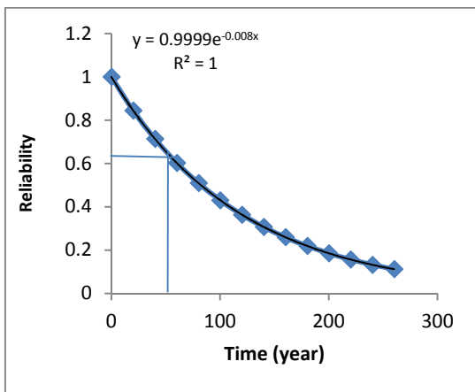
Fig 1: Reliability of Apa timber
