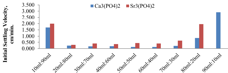
Fig 2: Effect of M/P (volume) ratio on precipitate initial settling velocity.
