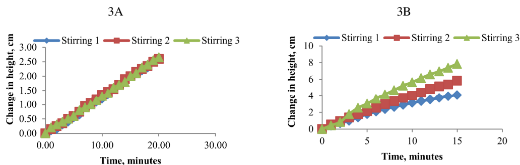
Fig 3: Residence time taken for (A) TCDP and (B) TSDP precipitates, at 30:70ml and 20:80ml (M/P) volume ratios.
