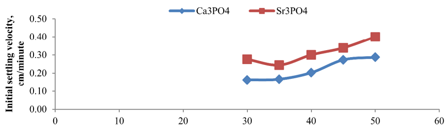
Fig 4: Initial settling velocity against temperature for TCDP and TSDP.
