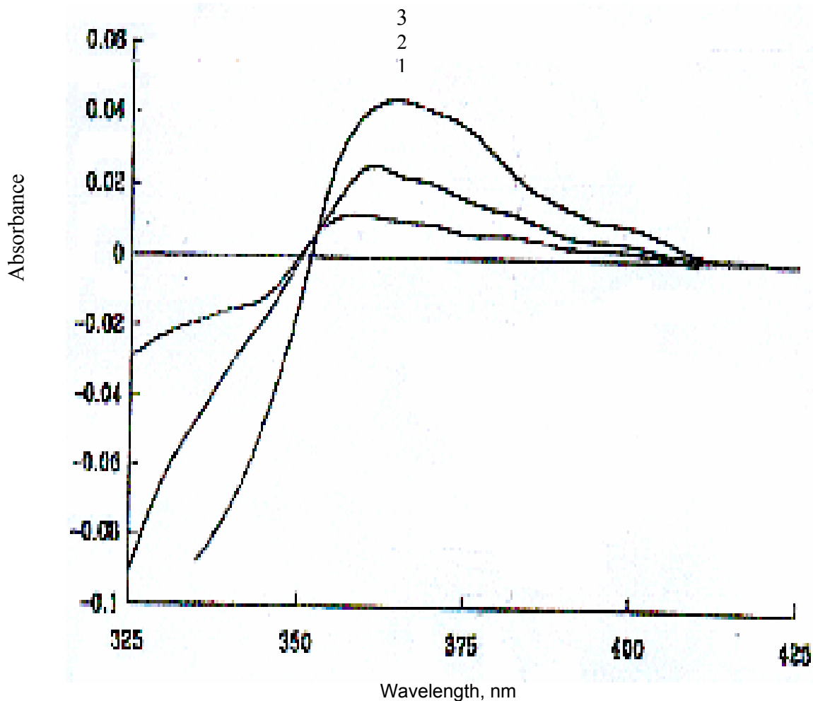
Fig. 1: Second order derivative spectra of Nickel (II)-KBAT against blank Conditions: Ni (II) \mu\text{g mL}^{-1} : 1 = 1.172, 2 = 1.758, 3 = 2.344, pH = 9.5
