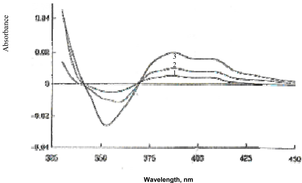
Fig. 2: Second order derivative spectra of Cobalt (II)-KBAT against blank Conditions: Co (II) \mu\text{g mL}^{-1} : 1 = 1.172, 2 = 1.779, 3 = 2.360, pH = 9.5
