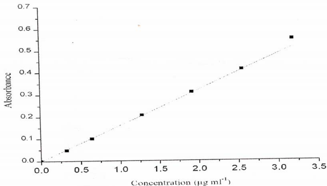
Fig. 3: Calibration graph for Ni (II) - KBAT complex by second derivative spectrum \lambda = 369.8 \text{ nm} , \text{pH} = 9.5
