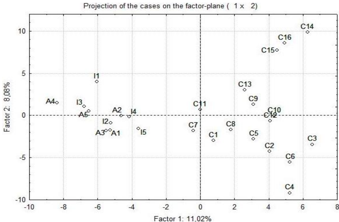
Figure 5. The resulting projection of principal component analysis.
