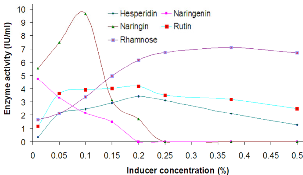
Figure 2. Effect of different concentration of inducers on enzyme production. Reaction conditions: pH 4.5, inoculum age 72 h, inoculum size 15%, temperature 27°C and agitation 200 rpm. Hesperidin, Naringenin, Naringin, Rutin and Rhamnose and their respective fermentation days are 5, 8, 7, 8 and 7.
