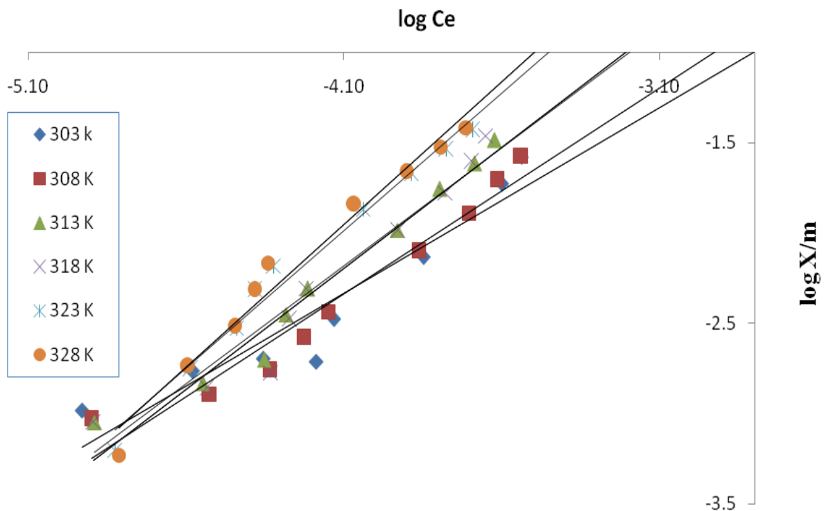
Figure 7. Freundlich isotherm plots of chitosan-rice husk (CRH) system and reactive red 195 (RR195).
