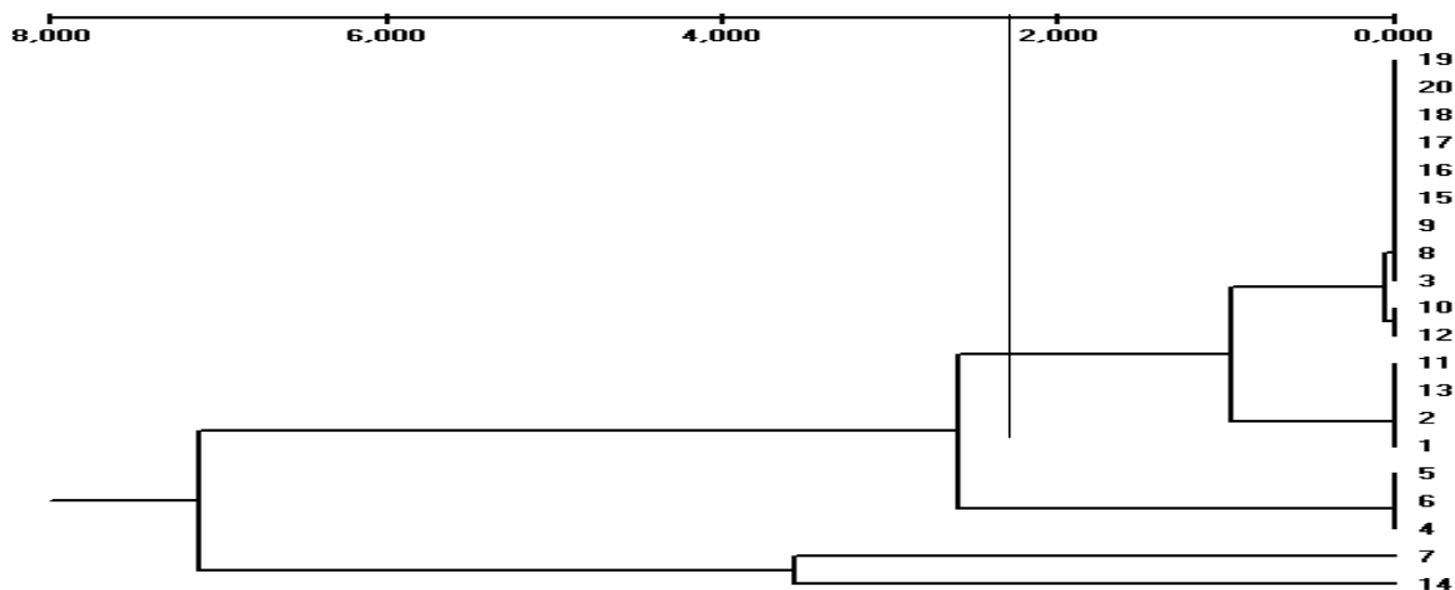
Figure 2. Dendrogram of 20 barley genotypes constructed based on Hordein bands. 1, 202799; 2, Arusigebs; 3, 225241; 4, 202802; 5, 202793; 6, 217125; 7, 217119; 8, 217126; 9, 202813; 10, Anbedat; 11, Enat gebs; 12, Workye; 13, Temaj; 14, Nechita; 15, Wogera; 16, Shedho; 17, Estaysh; 18, Trit; 19, Agegnhu; 20, Yedogit.
