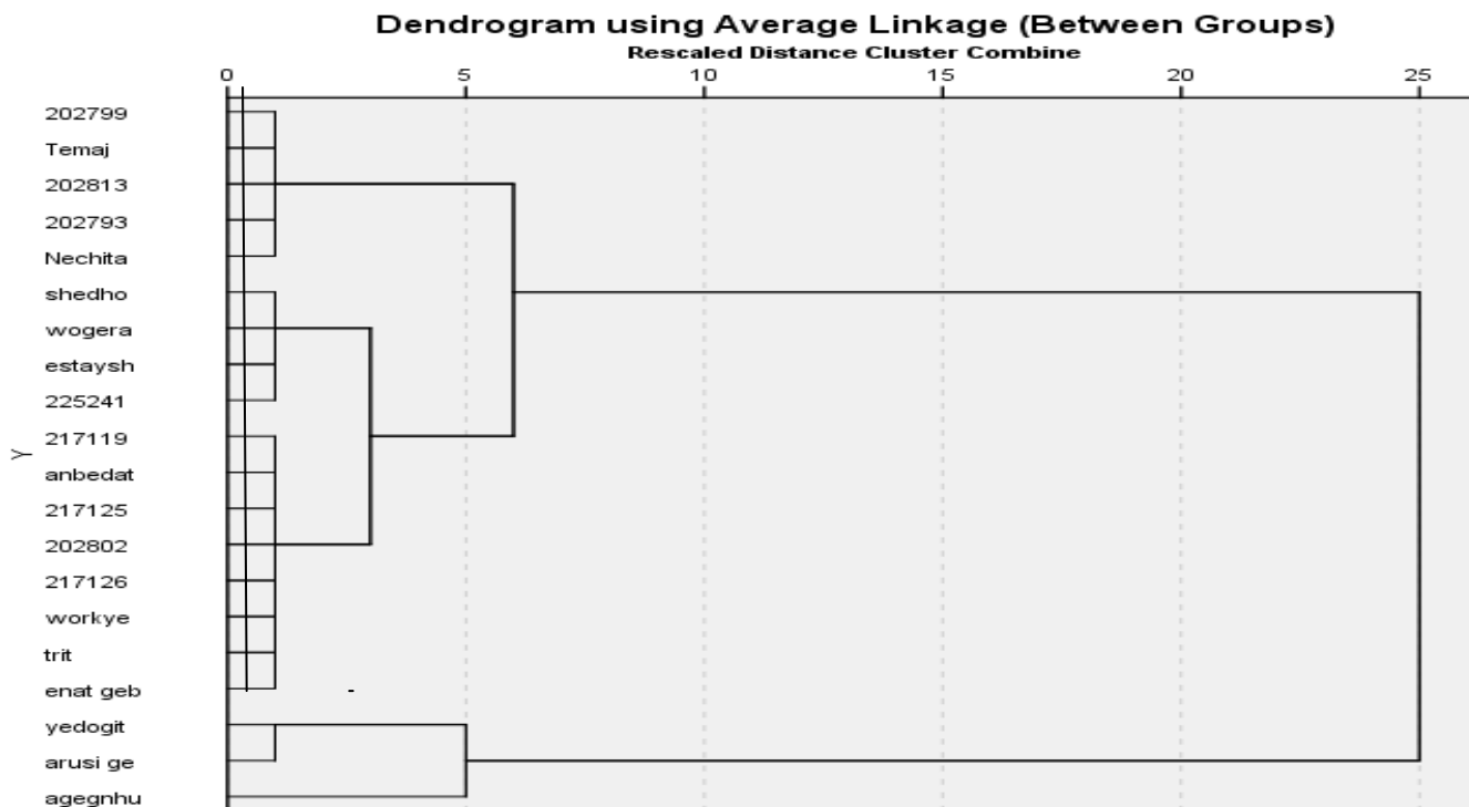
Figure 1. Dendrogram of barley genotypes constructed using agro-morphological traits.
