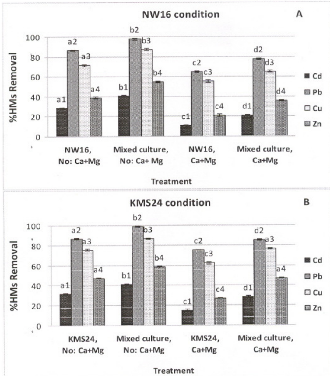
Figure 1. The heavy metals removal efficiency in the synthetic solution (Cd, 0.75 mg/L; Pb, 62.63 mg/L; Cu 34.60 mg/L; Zn, 58.50 mg/L) containing 3% NaCl in the presence or absence of 85 mg/L \text{Ca}^{2+} and 160 mg/L \text{Mg}^{2+} under aerobic-dark conditions by (A) pure culture of 4.5 mg DCW/ml of NW16 and the mixed of NW16 and KMS24 (2.5 + 2.5 mg DCW/ml) under optimum conditions for removal of HMs of NW16; pH 6.0, 30°C, 30 min and (B) pure culture of 5.0 mg DCW/ml of KMS24 and the mixed culture under optimum conditions for removal of HMs of KMS24; pH 5.5, 35°C, 45 min. Lower case letters with numbers above bars (that is, a1, b1, c1 and d1) using different letters indicate significant differences ( p < 0.05 ).
