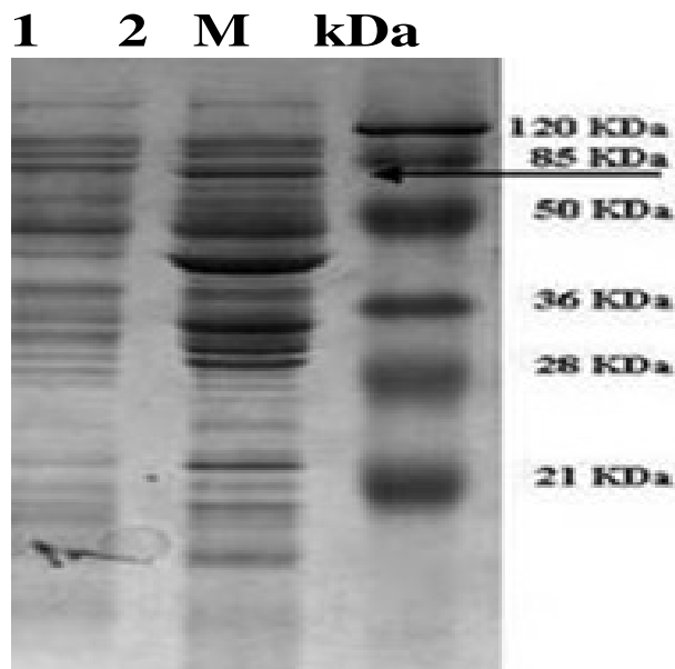
Figure 1. Expression of the recombinant CotA in E. coli . M, molecular weight markers Lane 1, supernatant of a crude extract of an uninduced E. coli BL21(DE3) culture; Lane 2, supernatant of a crude extract of an IPTG-induced E. coli BL21(DE3) culture. The band indicated by the arrow is the CotA protein.
