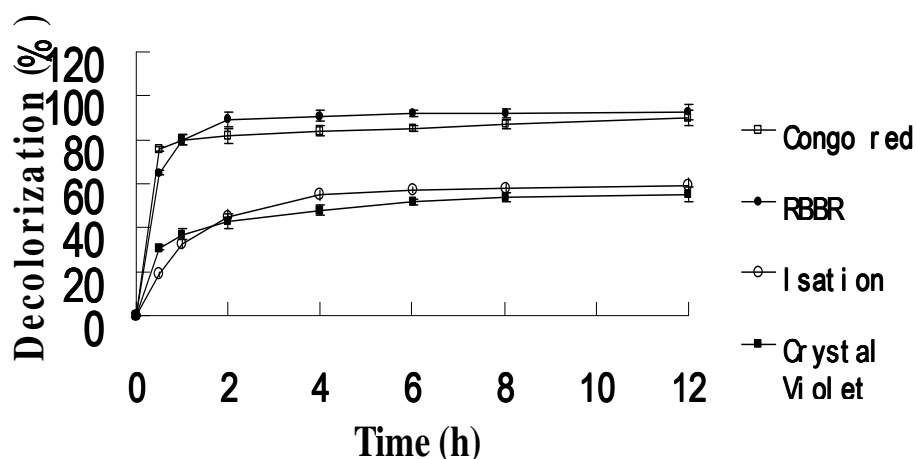
Figure 5. Decolorization of dyes with purified CotA laccase from E. coli .
