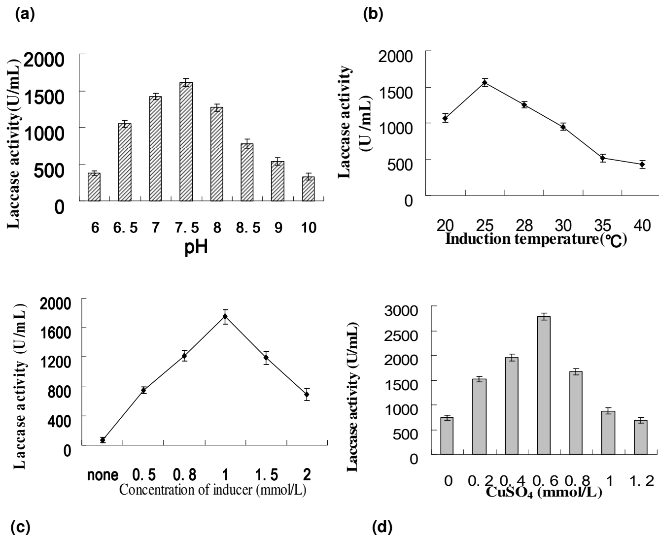
Figure 2. Effects of pH; a Induce temperature; b IPTG concentration; c and copper concentration; d on the production of laccase in LB medium supplemented with 0.2 mmol/L CuSO 4 . Cultivation conditions; a 0.2 mmol/L CuSO 4 , 1 mmol/L IPTG, 30°C; b 0.2 mmol/L CuSO 4 , pH 7, 30°C; c 0.2 mmol/L CuSO 4 , 1 mmol/L IPTG, 30°C; d 1 mmol/L IPTG, pH 7, 30°C.
