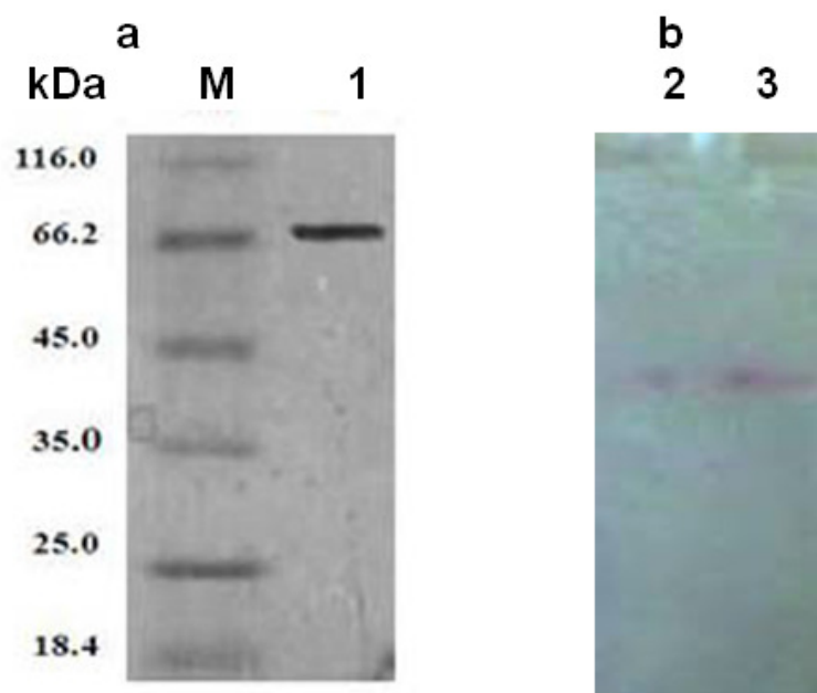
Figure 3. The SDS-PAGE result of the purified CotA protein: SDS-polyacrylamide gel analysis of CotA purified from recombinant E. coli BL21 (DE3). Samples of purified CotA were incubated for 5 min at 100°C (lane 1) before electrophoresis. The Native-PAGE result of the purified CotA protein was stained with syringaldazine (lane 2 and 3).
