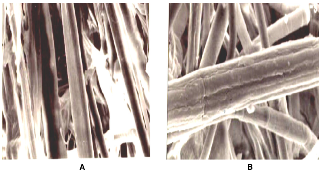
Figure 3. Scanning electron micrograph of (A) boiled mannanase treated (B) activated mannanase treated samples of wheat straw rich-soda pulp.
