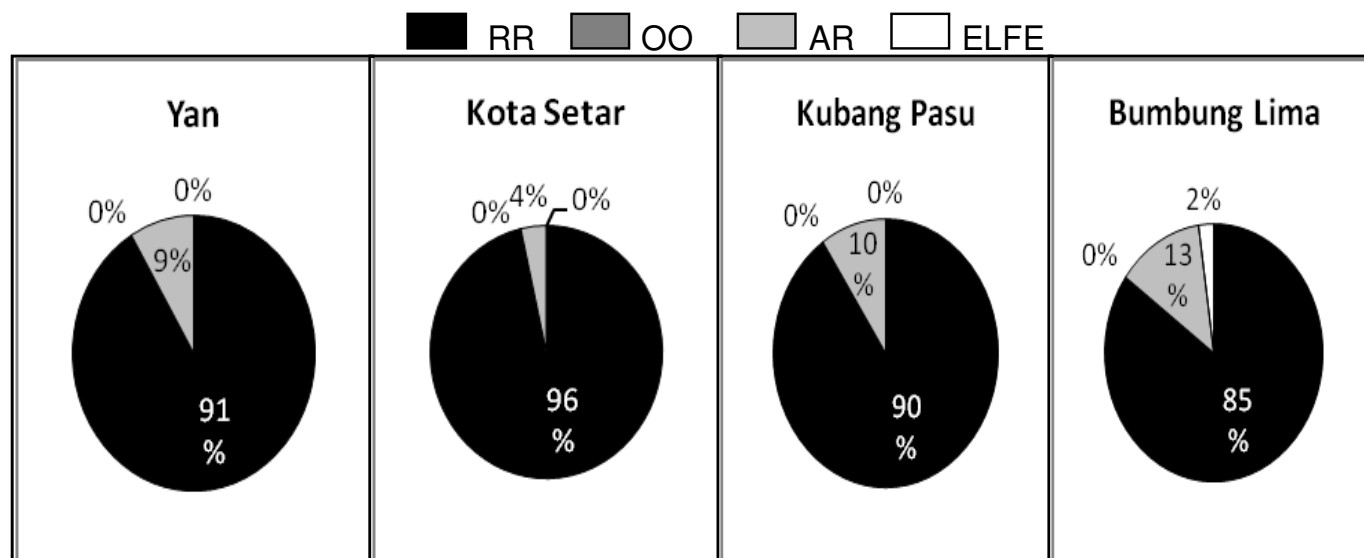
Figure 5. Speciation of Zn in paddy soils of Yan, Kota Setar, Kubang Pasu and Bumbung Lima.
