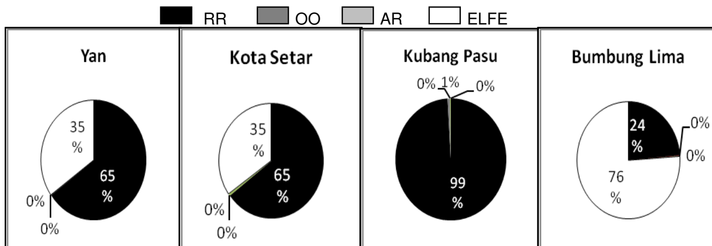
Figure 3. Speciation of Cd in paddy soils of Yan, Kota Setar, Kubang Pasu and Bumbung Lima.
