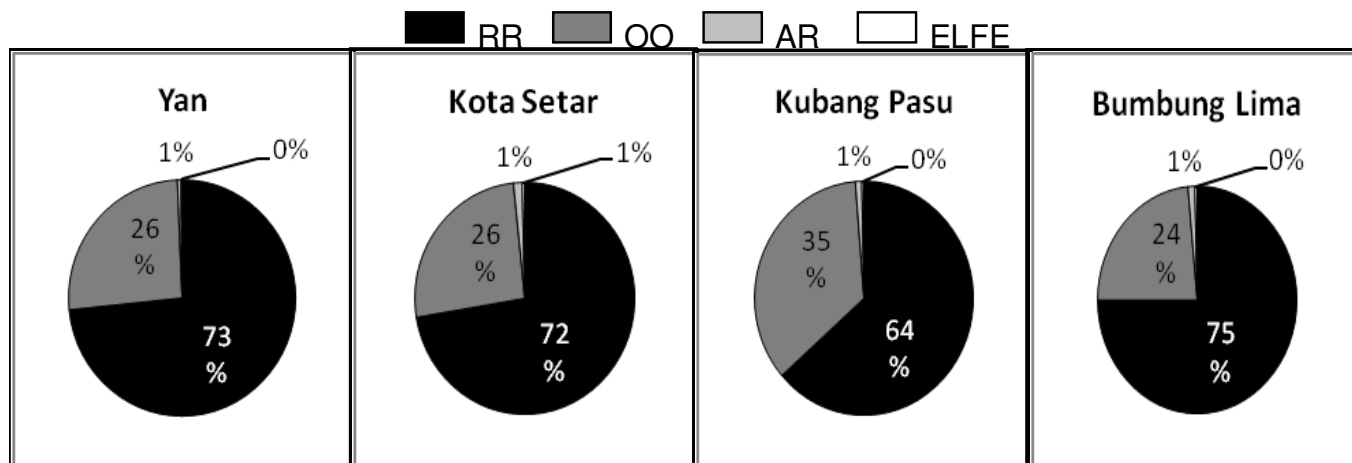
Figure 6. Speciation of Cr in paddy soils of Yan, Kota Setar, Kubang Pasu and Bumbang Lima.
