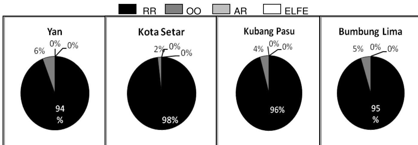
Figure 4. Speciation of Pb in paddy soils of Yan, Kota Setar, Kubang Pasu and Bumbung Lima.
