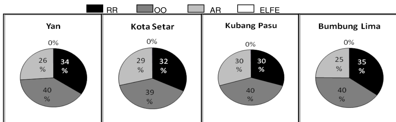
Figure 1. Speciation of Fe in paddy soils of Yan, Kota Setar, Kubang Pasu and Bumbung Lima.
