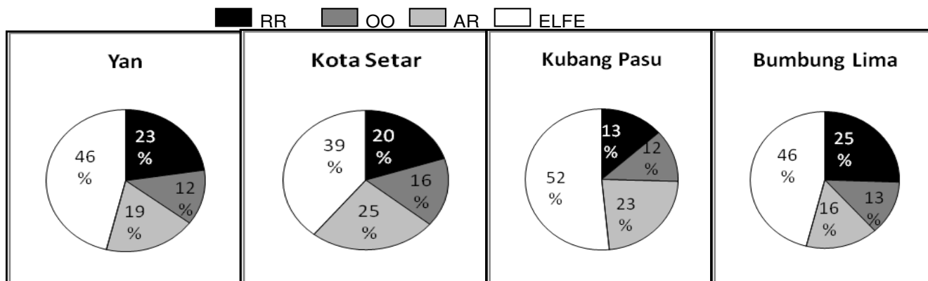
Figure 2. Speciation of Mn in paddy soils of Yan, Kota Setar, Kubang Pasu and Bumbung Lima.
