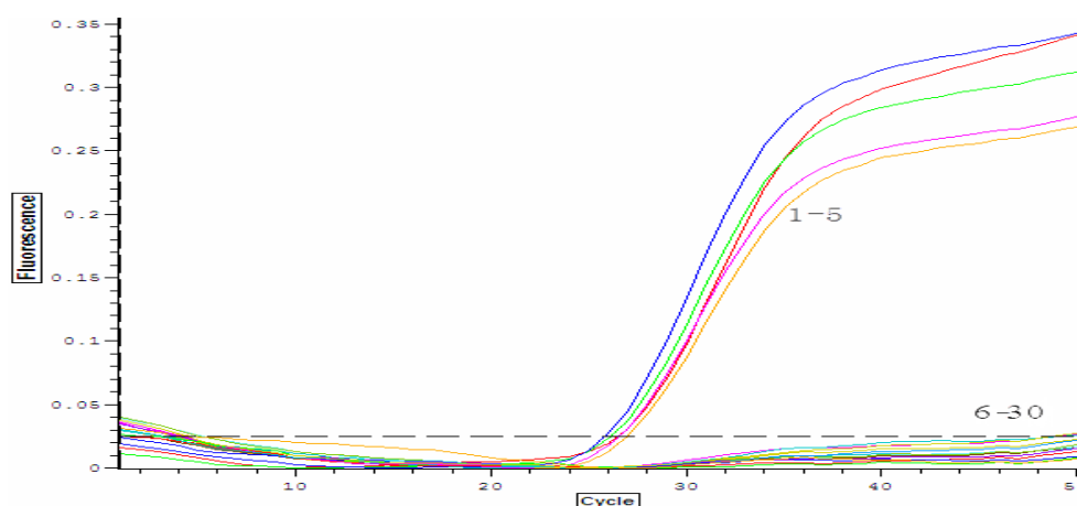
Figure 3. 1-5 are curves of Bifidobacterium ; 6-30 are curves of Lactobacillus , bacillus , salmonella , E. coli , S. aureus and Streptococcus (the strains were shown in Table 3).
