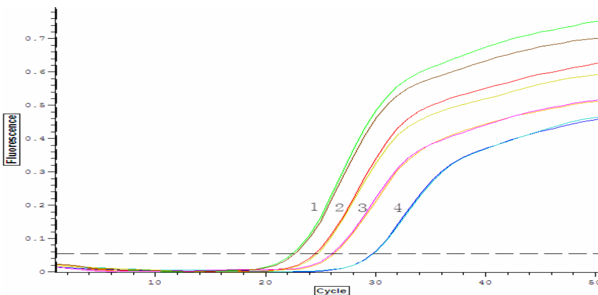
Figure 2. The values of two repeats of four different were showed to prove the reproducibility of developed real-time quantitative PCR.
